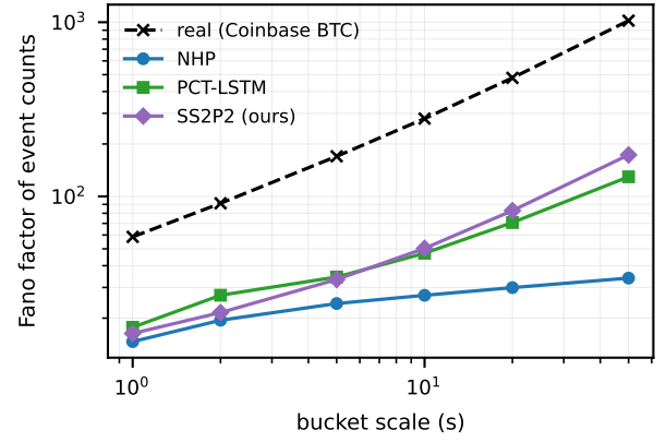
Figure 3: Fano factor of simulated event counts vs. bucket scale (Coinbase BTC; mean over calibrated checkpoints and roll-out seeds). Real order flow is super-Poissonian with Fano rising in scale; all models under-disperse at this context length, SS2P2 and PCT-LSTM least.
