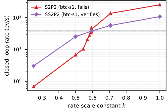
Figure 4: Calibration probe ladders on BTC (target band shaded): the failing S2P2 checkpoint’s closed-loop rate is near-discontinuous in the rescaling constant \kappa ; the verified SS2P2 checkpoint crosses the target smoothly.
