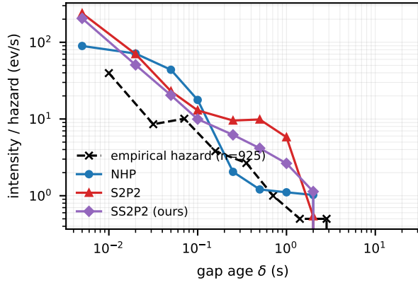
Figure 2: Mean model intensity at gap age \delta , among BTC test gaps that survive past \delta , vs. the empirical hazard of the real gap distribution (log-log; survivor counts shrink toward the right). NHP tracks the falling hazard; the state-space family stays hot through quiet gaps — the timeNLL gap of Table 1 accrues here.
