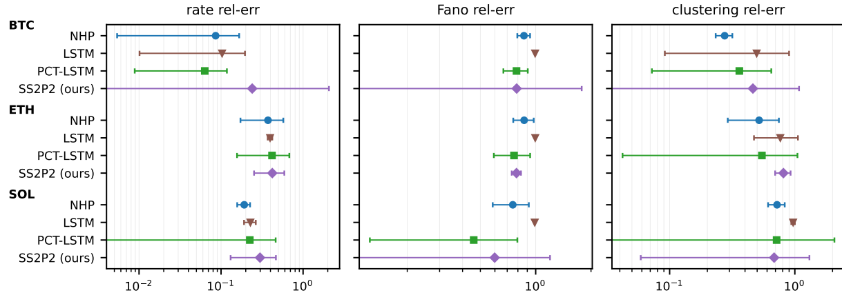
Figure 5: Simulation quality across assets (rel-err vs. real, log scale; whiskers = 95% CI over checkpoints). s2p2 and SAHP omitted where no calibrated checkpoints exist.
