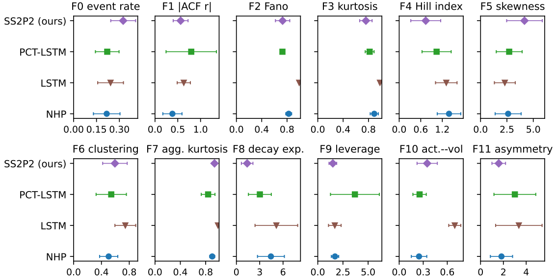
Figure 3: The full stylized-fact battery, pooled across the three assets: relative error vs. real for the twelve facts F0–F11: event rate (F0), Fano factor averaged over 1–50 s scales (F2), and the distributional facts (whiskers = 95% CI over asset-checkpoint pairs; roll-out seeds averaged within checkpoint). S2P2 and SAHP omitted: too few calibrated checkpoints.
