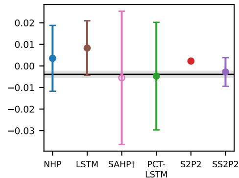
F11 timescale asymmetry (coarse \rightarrow fine, > 0 )
