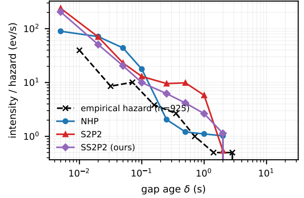
Figure 3: Mean model intensity at gap age \delta , among BTC test gaps that survive past \delta , vs. the empirical hazard of the real gap distribution (log-log; survivor counts shrink toward the right). NHP tracks the falling hazard; the state-space family stays hot through quiet gaps — the timeNLL gap of Table 1 accrues here.
