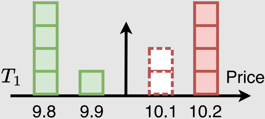
Market order
