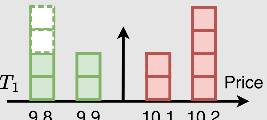
Cancel order
