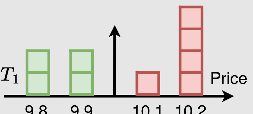
Limit order
