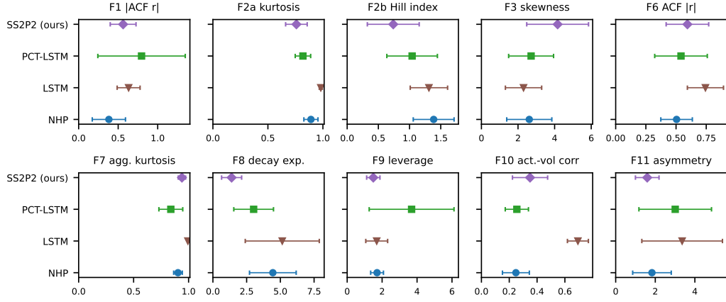
Figure 4: All ten stylized facts, pooled across the three assets: relative error vs. real (whiskers = 95% CI over asset-checkpoint pairs; roll-out seeds averaged within checkpoint). S2P2 and SAHP omitted: too few calibrated checkpoints.
