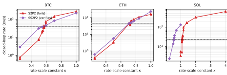
Figure 6: Calibration probe ladders on all three assets (target band shaded, seed-1 checkpoints): the failing S2P2 checkpoints’ closed-loop rates are near-discontinuous in the rescaling constant \kappa , most extremely on SOL; the verified SS2P2 checkpoints cross each target smoothly.
