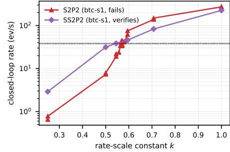
Figure 6: Calibration probe ladders on BTC (target band shaded): the failing S2P2 checkpoint’s closed-loop rate is near-discontinuous in the rescaling constant \kappa ; the verified SS2P2 checkpoint crosses the target smoothly.
