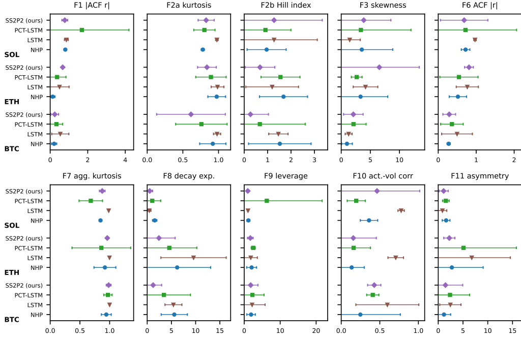
Figure 4: All ten stylized facts across assets: relative error vs. real (whiskers = 95% CI over checkpoints; roll-out seeds averaged within checkpoint). S2P2 and SAHP omitted where no calibrated checkpoints exist.
