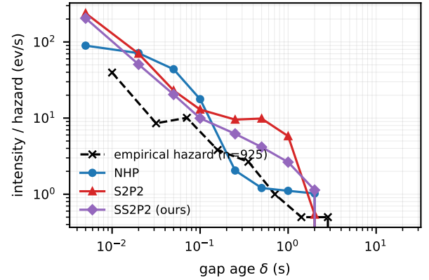
Figure 1: Mean model intensity at gap age \delta , among BTC test gaps that survive past \delta , vs. the empirical hazard of the real gap distribution (log-log; survivor counts shrink toward the right). NHP tracks the falling hazard; the state-space family stays hot through quiet gaps — the timeNLL gap of Table 1 accrues here.
