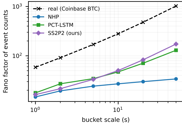
Figure 2: Fano factor of simulated event counts vs. bucket scale (Coinbase BTC; mean over calibrated checkpoints and roll-out seeds). Real order flow is super-Poissonian with Fano rising in scale; all models under-disperse at this context length, SS2P2 and PCT-LSTM least.
