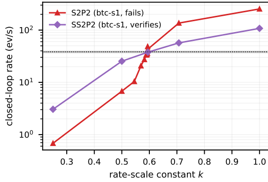
Figure 3: Calibration probe ladders on BTC (target band shaded): the failing S2P2 checkpoint’s closed-loop rate is near-discontinuous in the rescaling constant k ; the verified SS2P2 checkpoint crosses the target smoothly.
