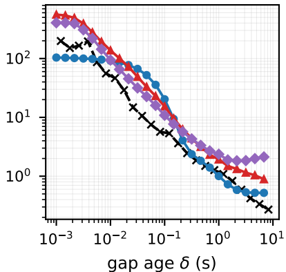
ETH
