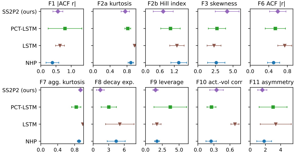
Figure 4: All ten stylized facts, pooled across the three assets: relative error vs. real (whiskers = 95% CI over asset-checkpoint pairs; roll-out seeds averaged within checkpoint). S2P2 and SAHP omitted: too few calibrated checkpoints.
