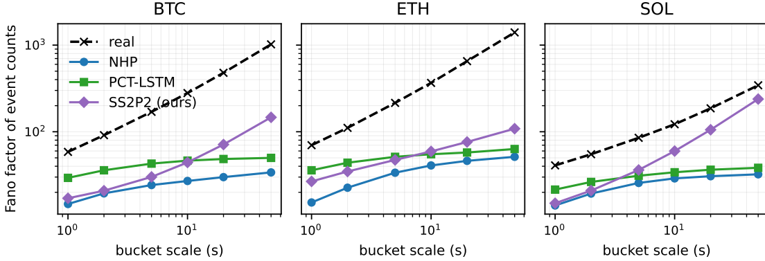
Figure 5: Real order flow is super-Poissonian with Fano rising in scale, and every model under-disperses at this context length, SS2P2 and PCT-LSTM least; the pattern is identical on all three assets. Curves are Fano factors of simulated event counts vs. bucket scale (mean over calibrated checkpoints and roll-out seeds).
