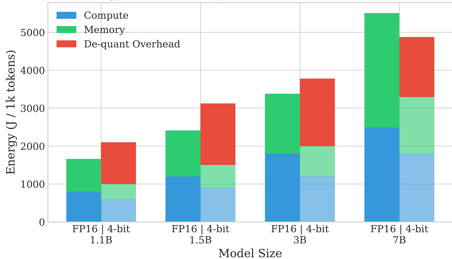
Energy Breakdown: Why Quantization Hurts Small Models
