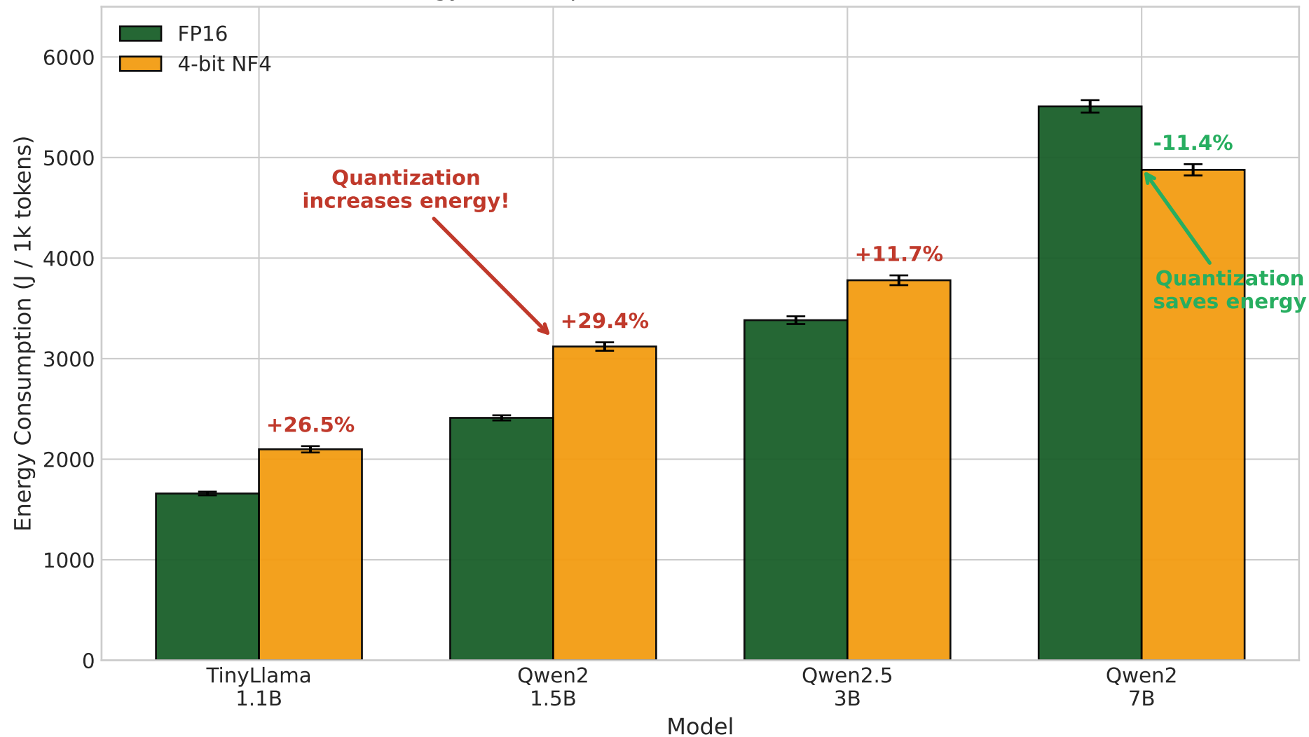
Energy Consumption: FP16 vs 4-bit NF4 on RTX 5090
