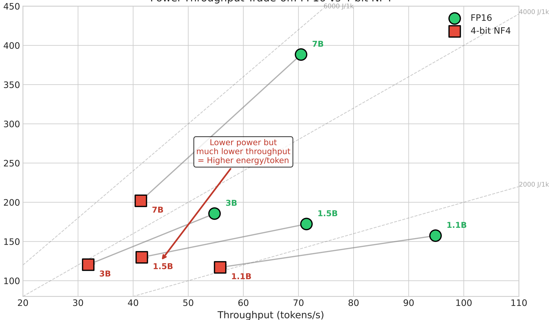
Power-Throughput Trade-off: FP16 vs 4-bit NF4
