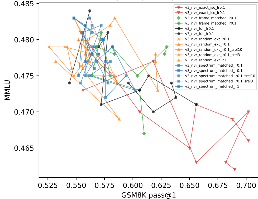
RLVR: trajectory (every 50 steps)
