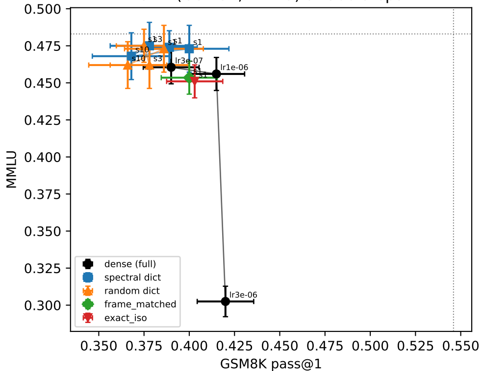
SFT: (GSM8K, MMLU) at 300 steps
