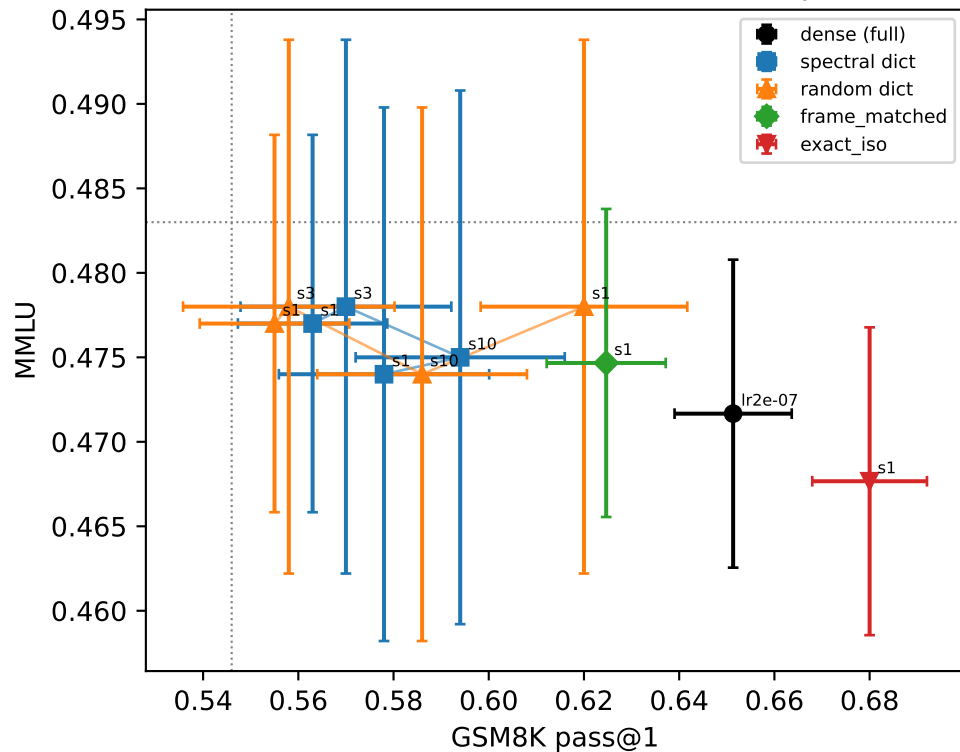
RLVR: (GSM8K, MMLU) at 300 steps
