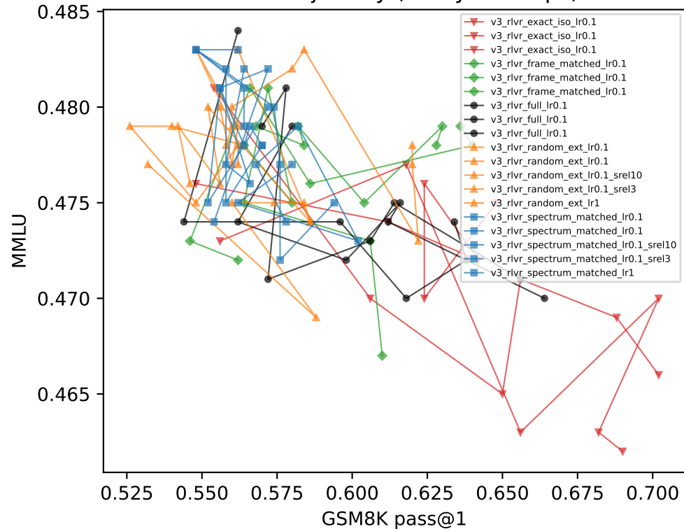
RLVR: trajectory (every 50 steps)
