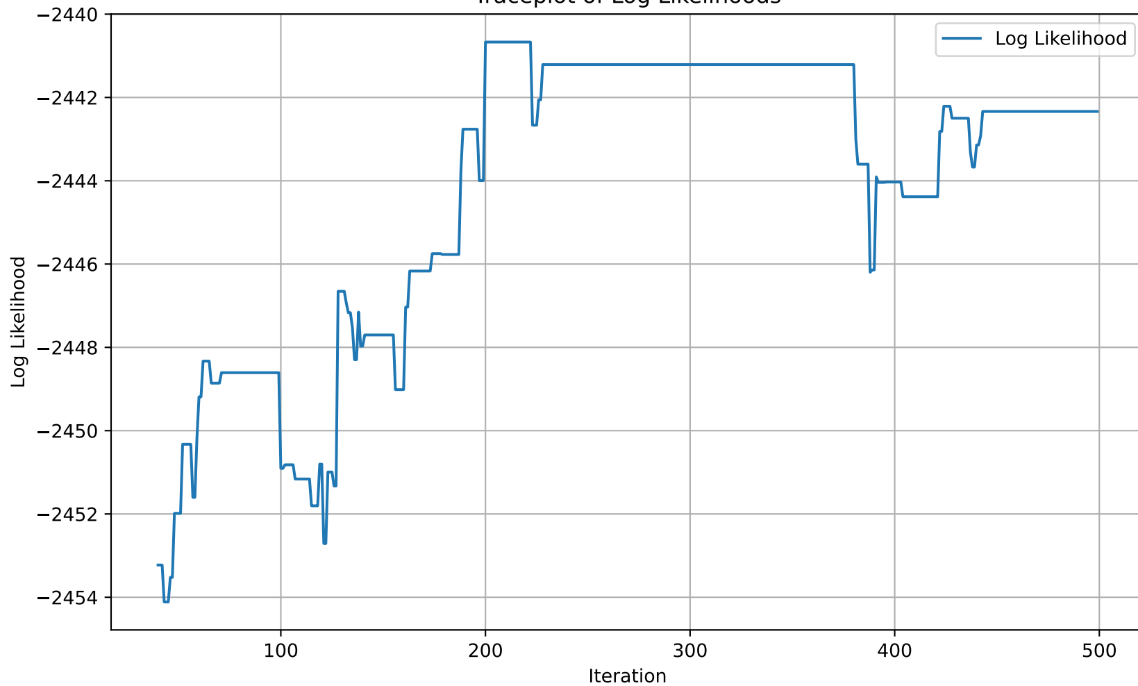
Traceplot of Log Likelihoods
