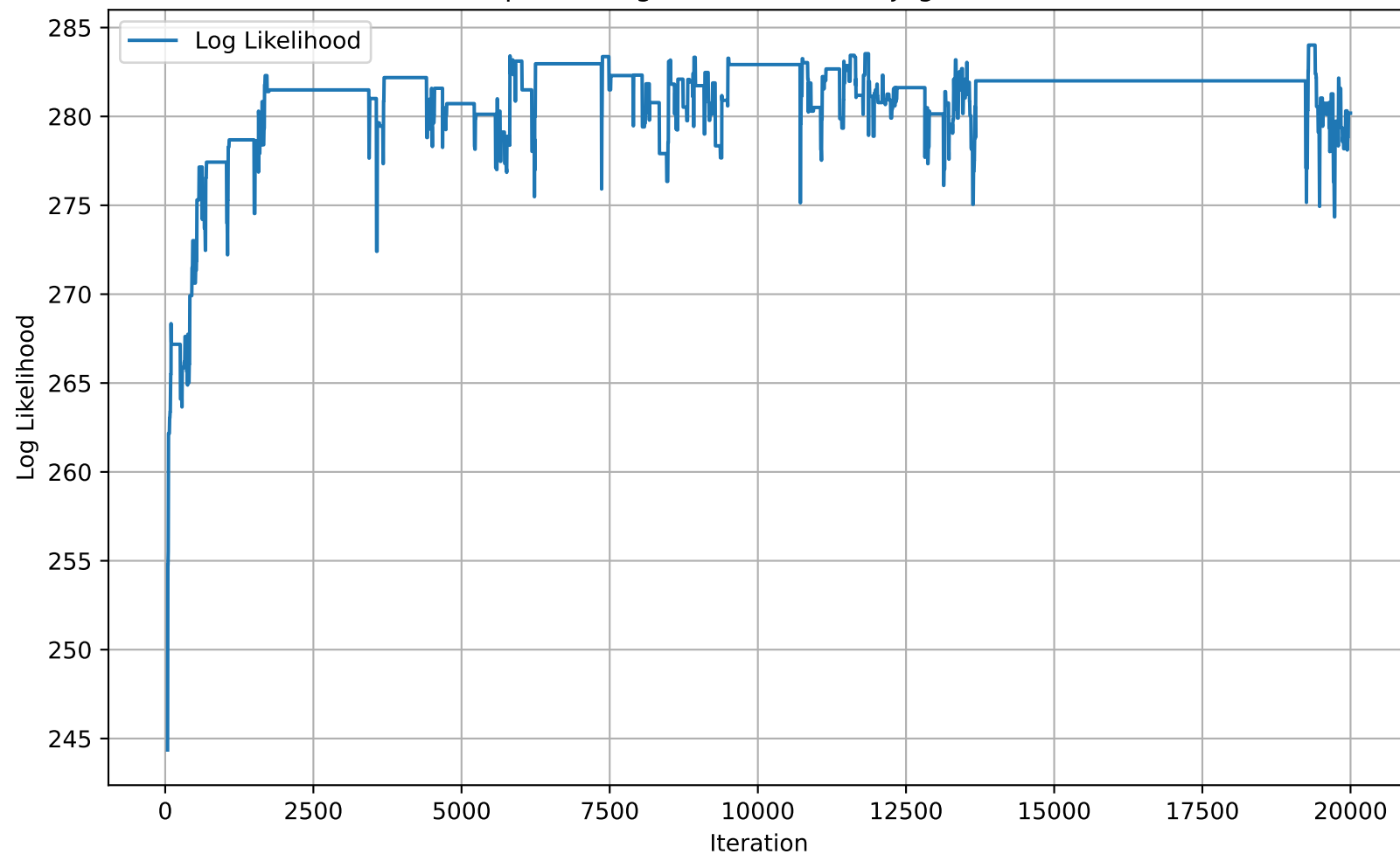
Traceplot of Log Likelihoods (Conjugate Priors)
