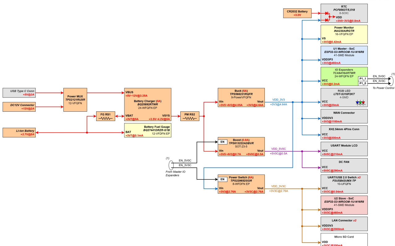
MODULAR IOT GATEWAY - POWER DIAGRAM Version 1
