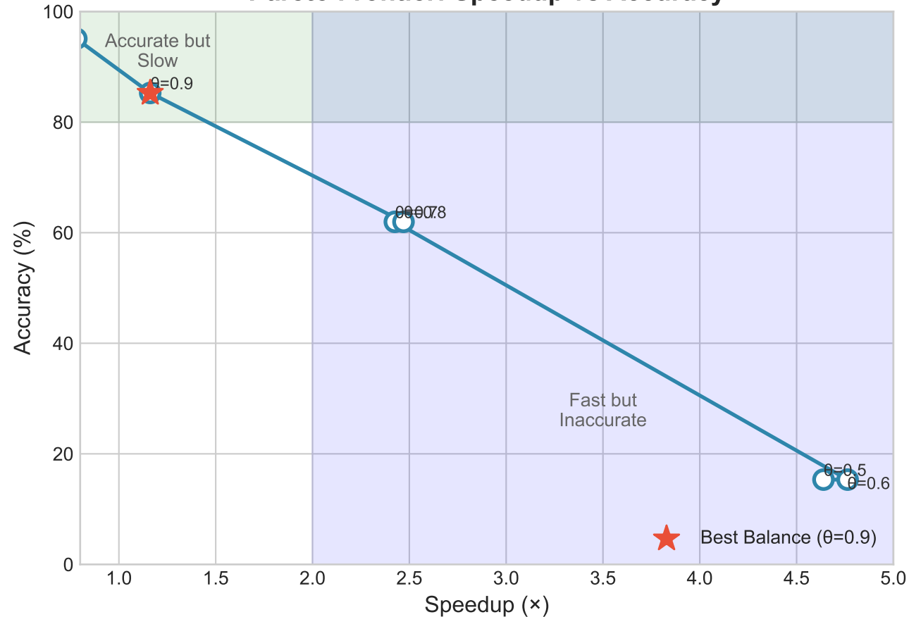
Pareto Frontier: Speedup vs Accuracy
