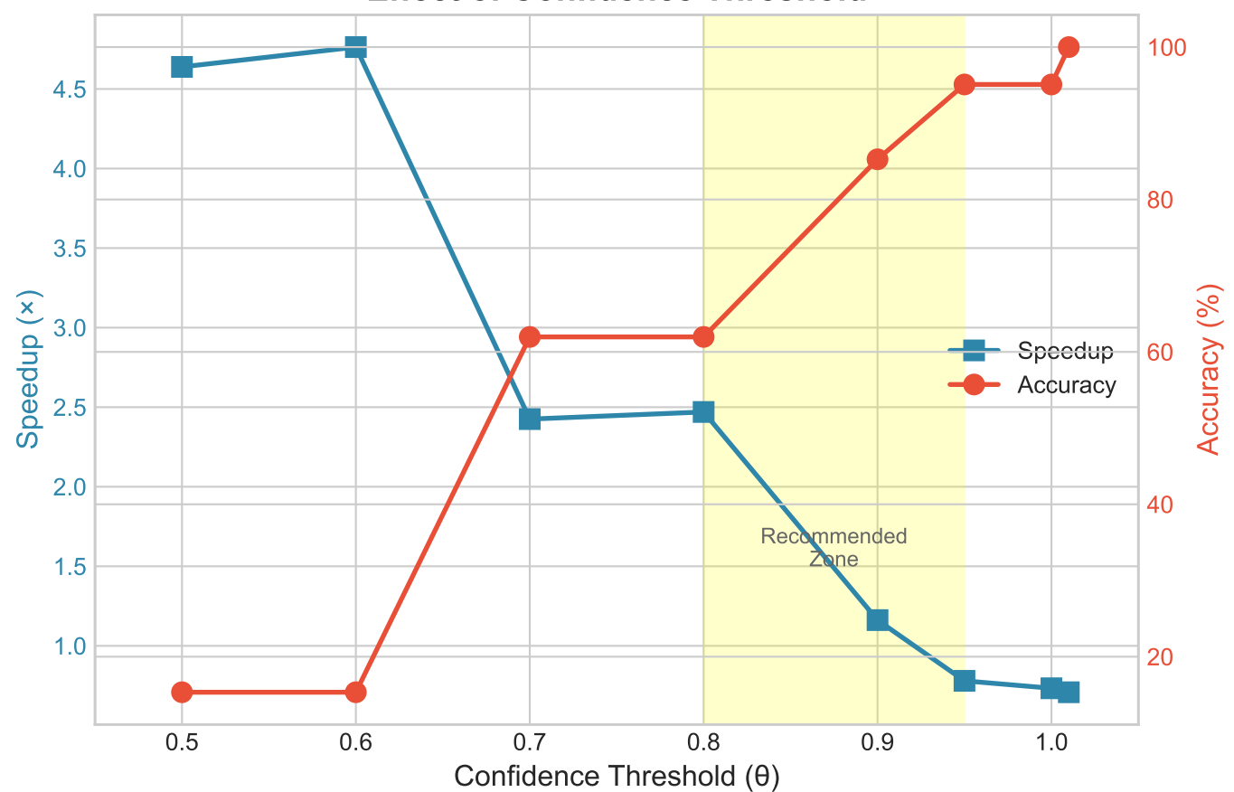
Effect of Confidence Threshold
