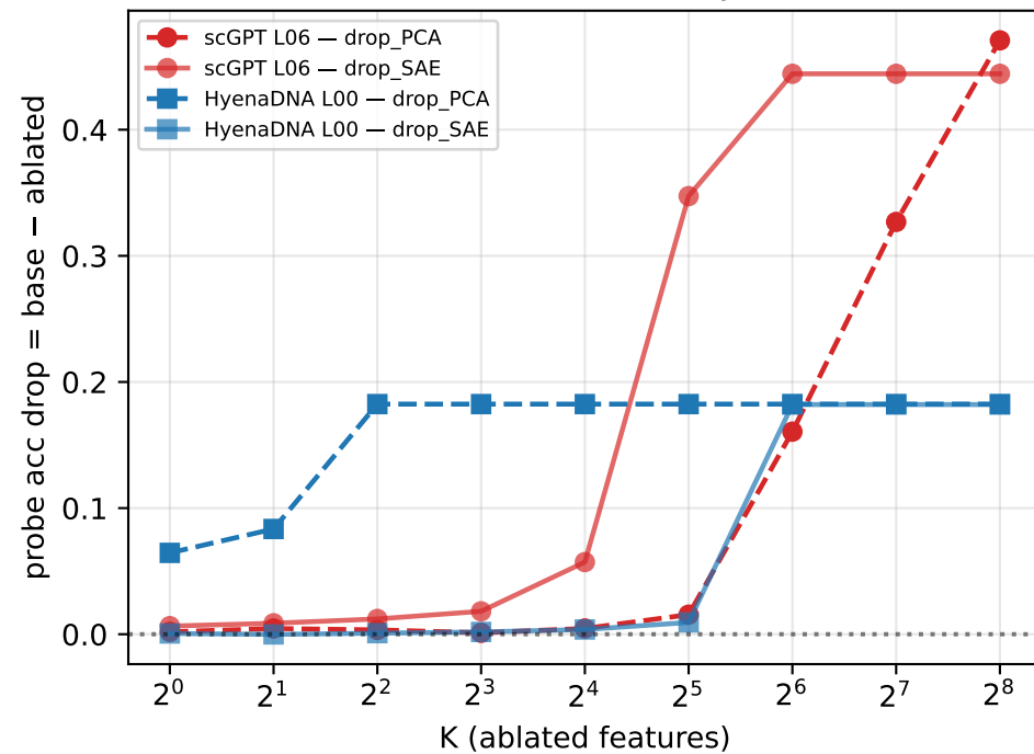
Decomposition: drop_PCA (dashed) vs drop_SAE (solid) for two 'extreme' layers
