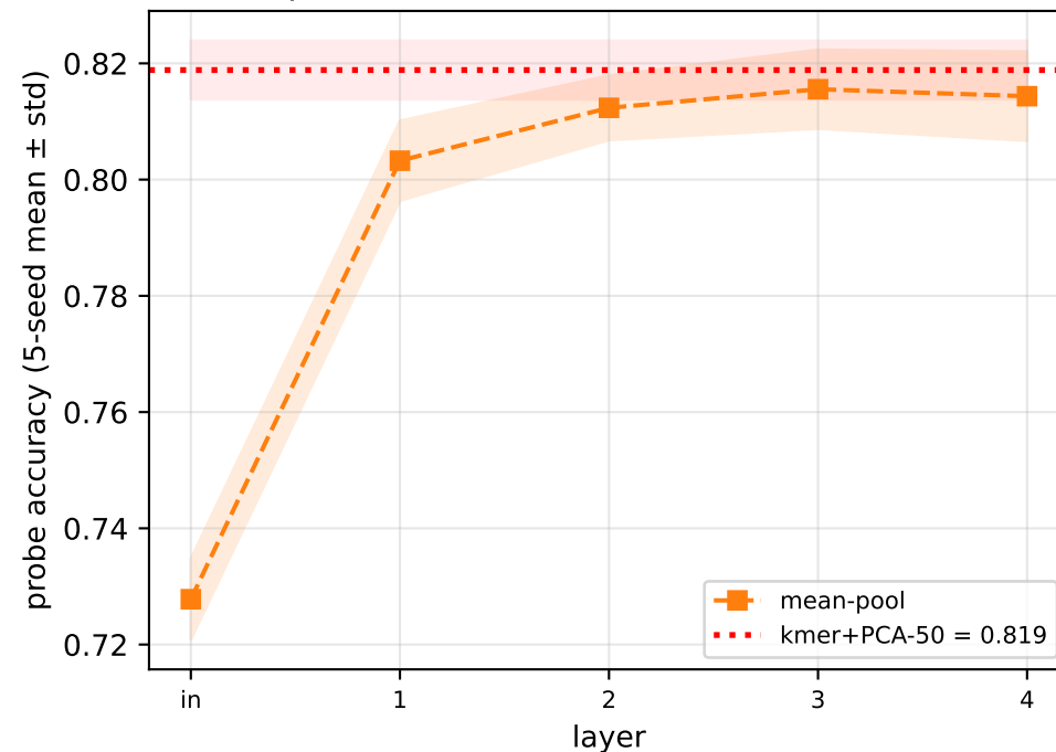
HyenaDNA × genomic_benchmarks probe acc vs kmer+PCA-50 baseline
