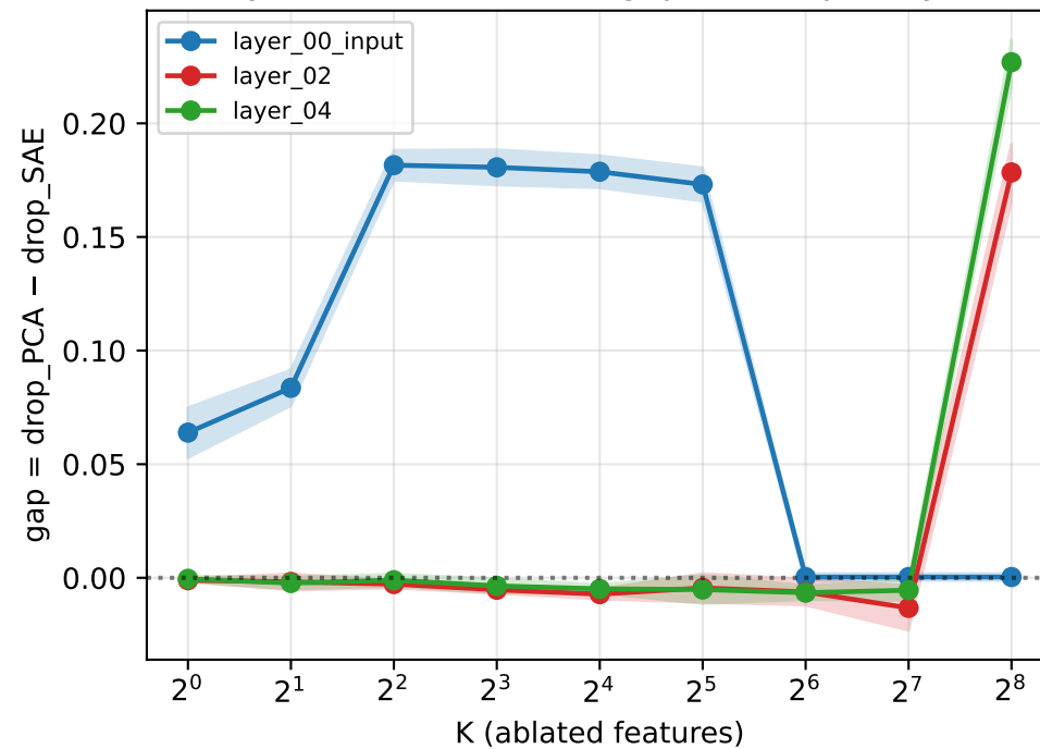
HyenaDNA — ablation gap curves per layer
