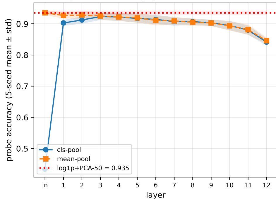
scGPT × pbmc3k probe acc vs log1p+PCA-50 baseline
