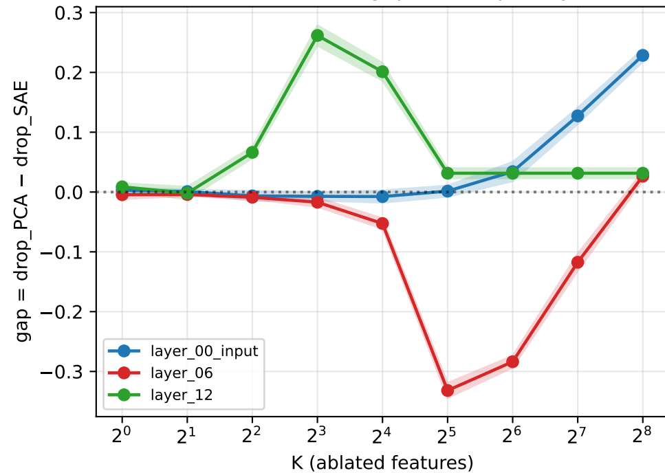
scGPT — ablation gap curves per layer
