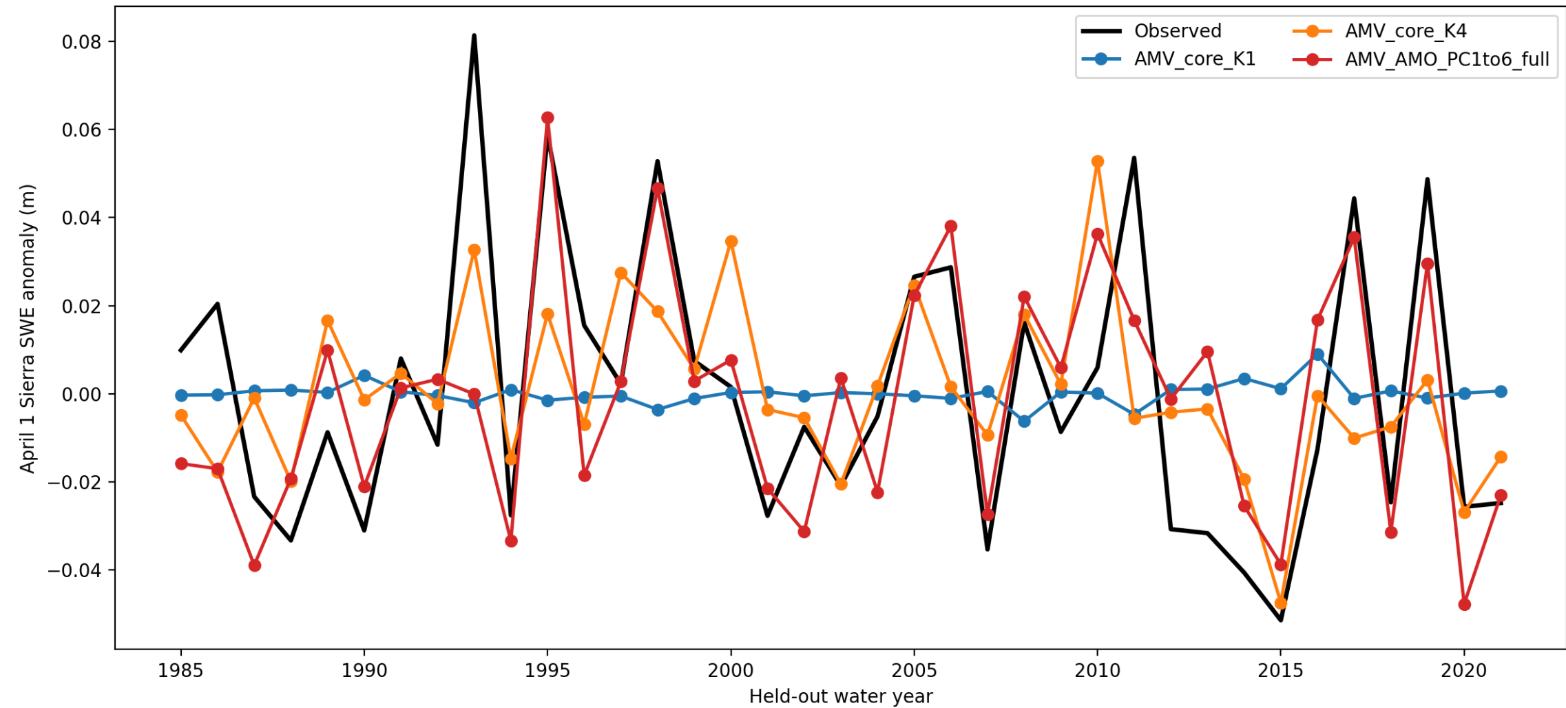
Observed vs predicted for fixed-core cumulative AMV/AMO models
