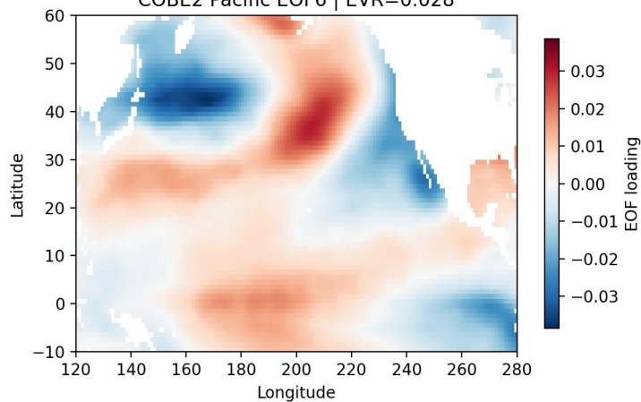
COBE2 Pacific EOF6 | EVR=0.028
