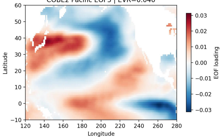
COBE2 Pacific EOF5 | EVR=0.040
