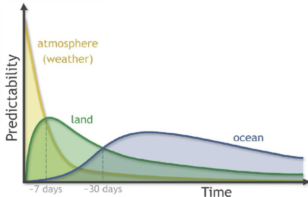
FIGURE: Relative contributions to Earth System predictability from the atmosphere, land, and ocean at different timescales.
