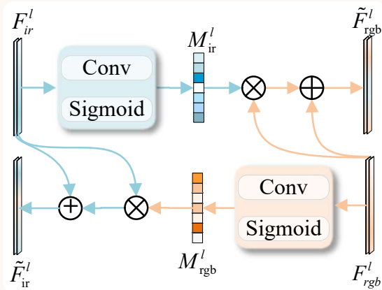
(a) Cross-Modal Saliency Interaction
