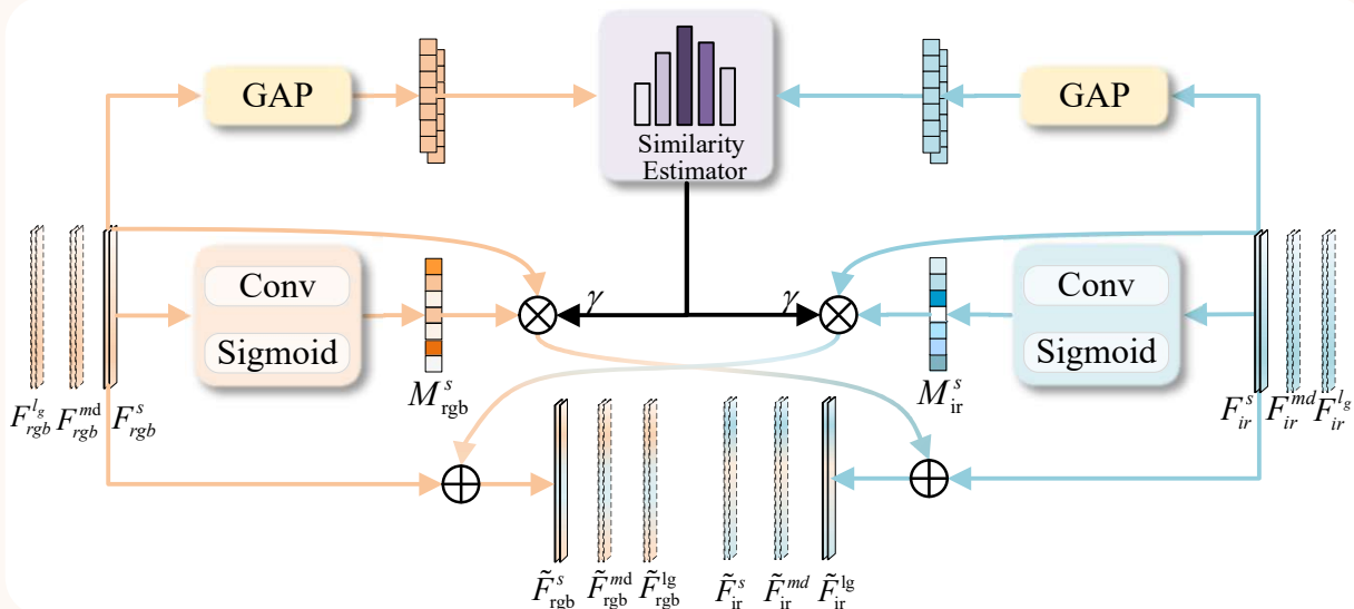
(b) Cross-Modal Similarity Interaction
