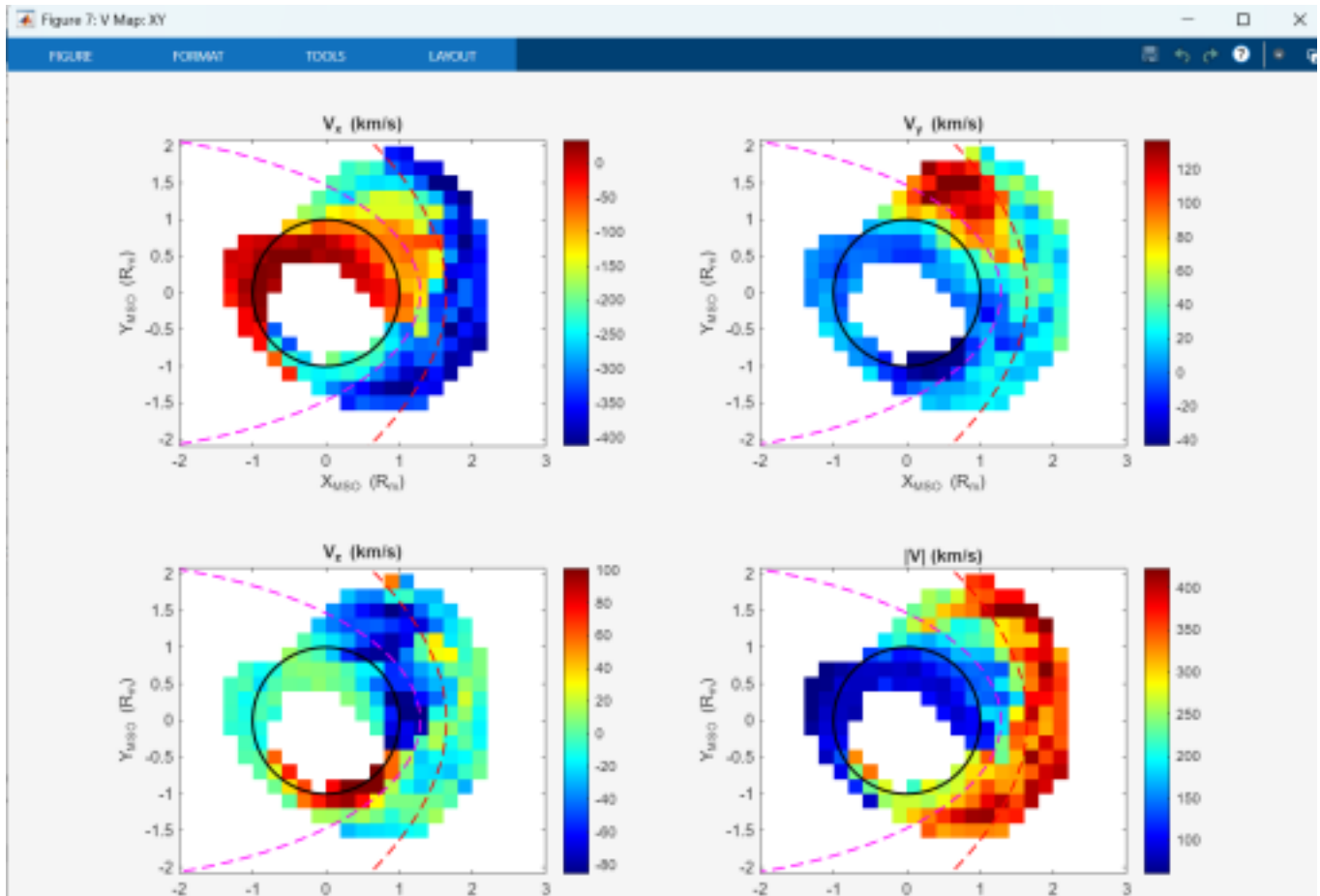
Velocity map in the XY plane, showing the velocity components ( V_x , V_y , V_z ) and total speed ( |V| ) in km/s.
