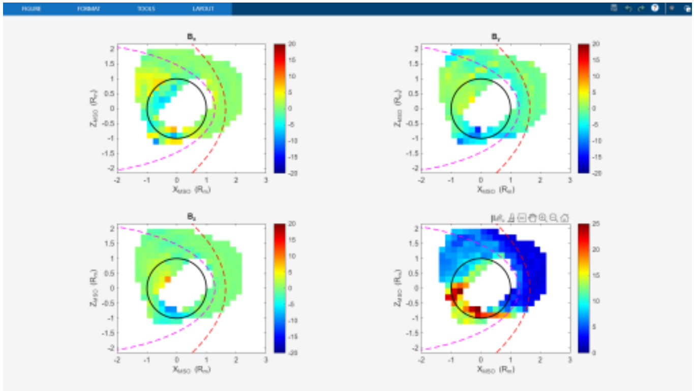
Magnetic field map in the XZ plane, showing the magnetic field components ( B_x , B_y , B_z ) and magnitude ( |B| ) in nT.
