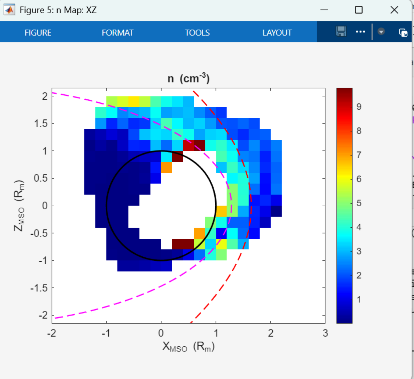
Proton density map in the XZ plane, with n ranging from approximately 1 to 9 \text{cm}^{-3} .
