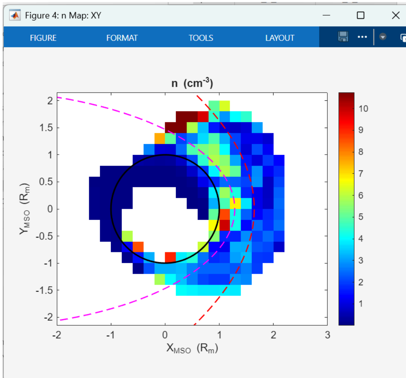
Proton density map in the XY plane, with n ranging from approximately 1 to 10 \text{ cm}^{-3} .
