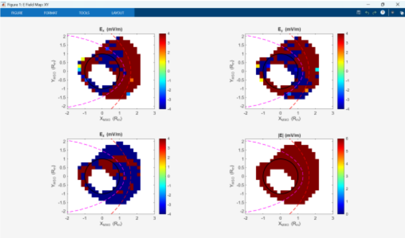
Convective electric field map in the XY plane, showing E_x , E_y , E_z and |E| in mV/m. Description matched to the
