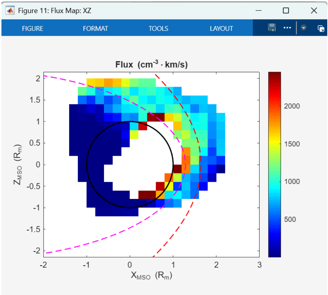
Ion flux map in the XZ plane, displaying the flux distribution along the noon–midnight meridian. Description
