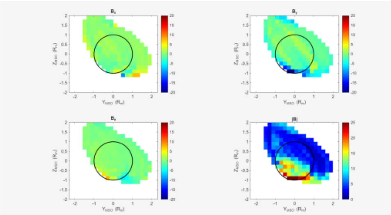
Magnetic field map in the YZ plane, showing the magnetic field components ( B_x , B_y , B_z ) and magnitude ( |B| ) in nT.
