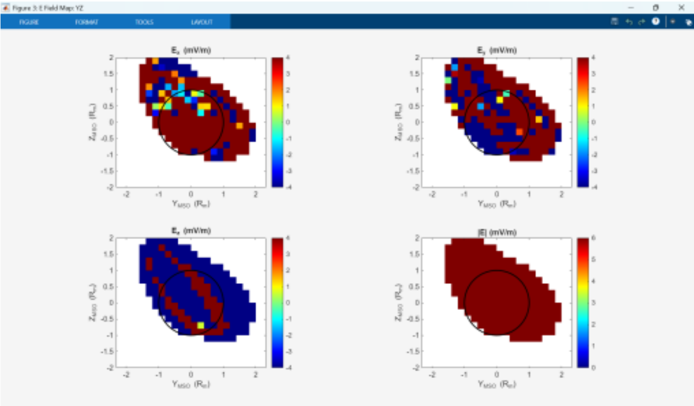
Convective electric field map in the YZ plane, showing E_x , E_y , E_z and |E| in mV/m. Description matched to the
