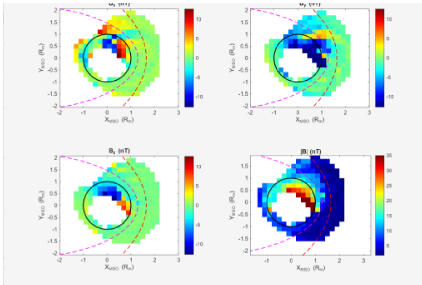
Magnetic field map in the XY plane, showing B_x , B_y , B_z and |B| in nT.
