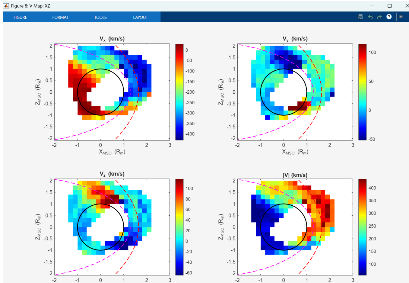
Velocity map in the XZ plane, showing V_x , V_y , V_z and |V| in km/s with boundary overlays. Description matched to
