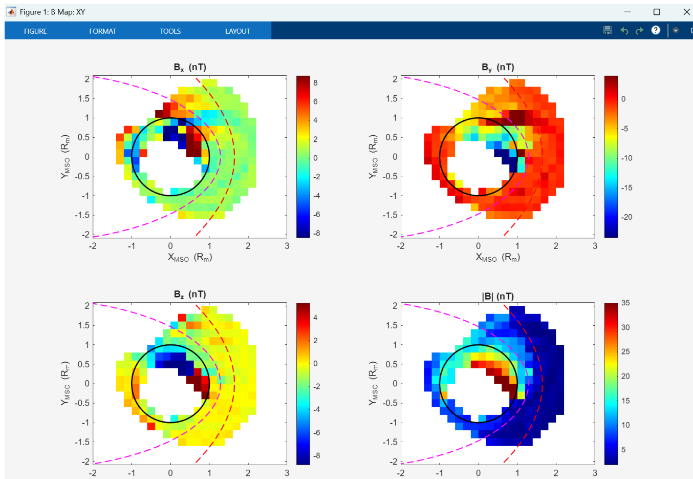
Magnetic field map in the XY plane, showing B_x , B_y , B_z and |B| in nT.
