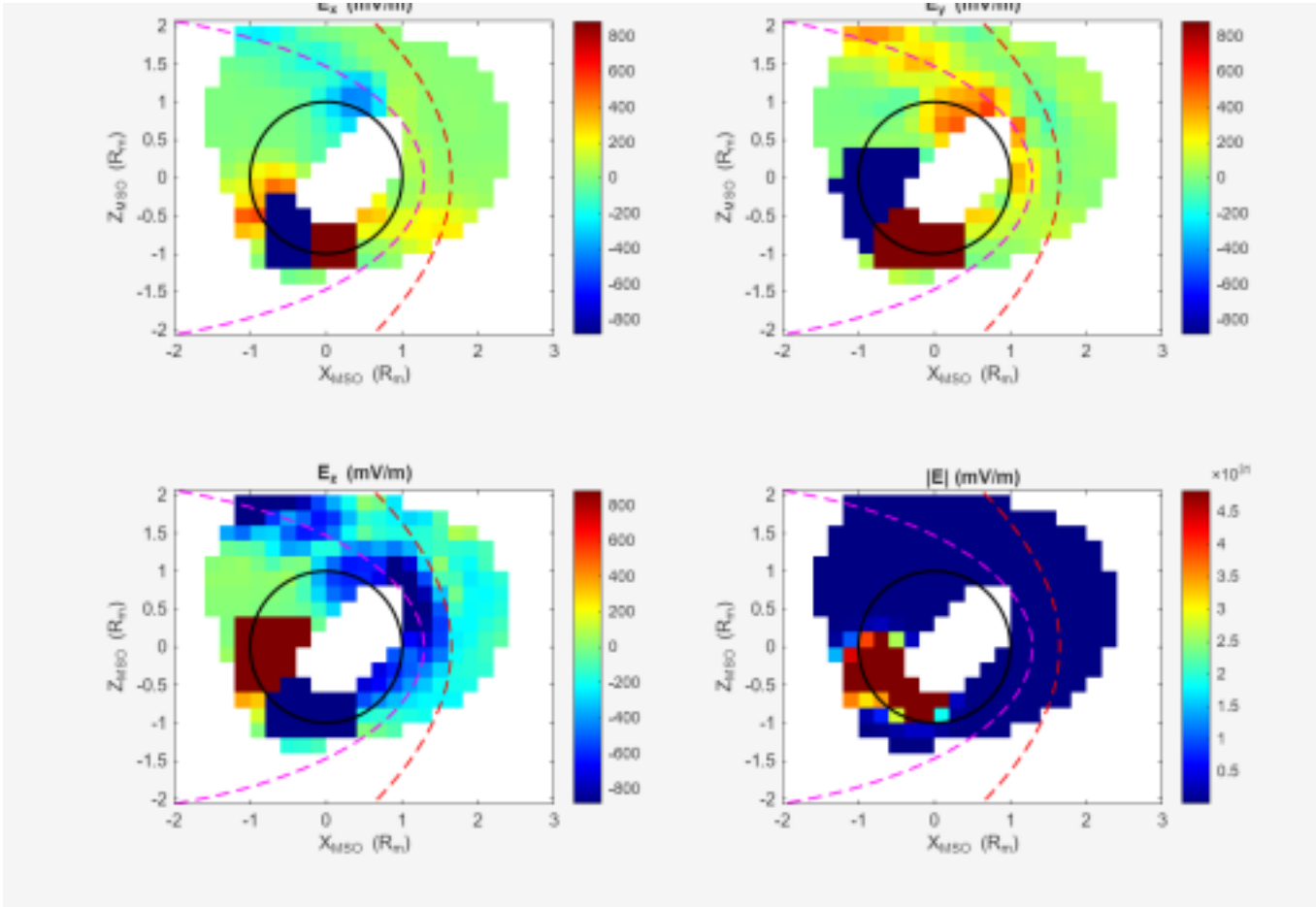
Convective electric field map in the XZ plane, showing E_x , E_y , E_z and |E| in mV/m. Description matched to the
