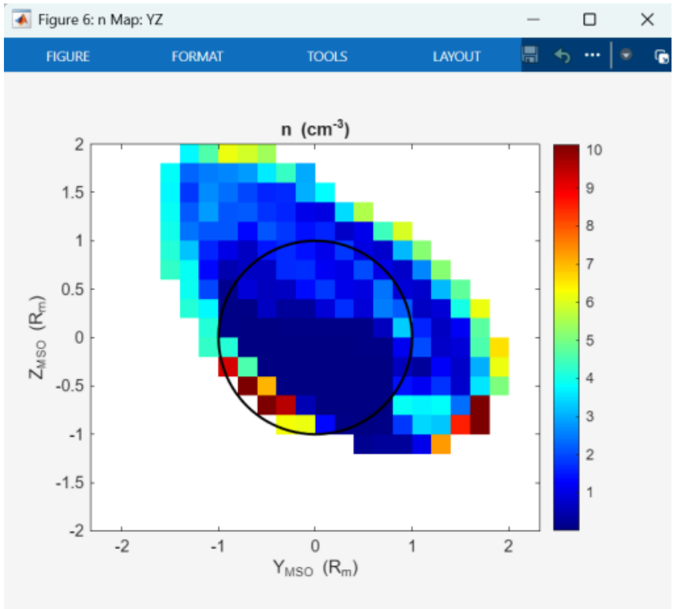
Ion density map in the YZ plane, showing the proton density distribution across the cross-tail projection.
