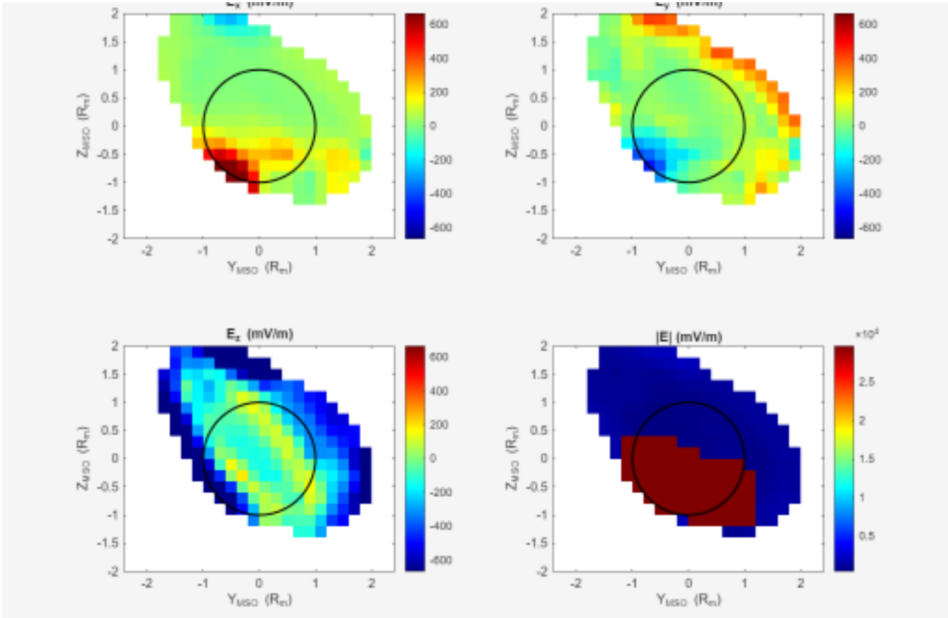
Convective electric field map in the YZ plane, showing E_x , E_y , E_z and |E| in mV/m. Description matched to the
