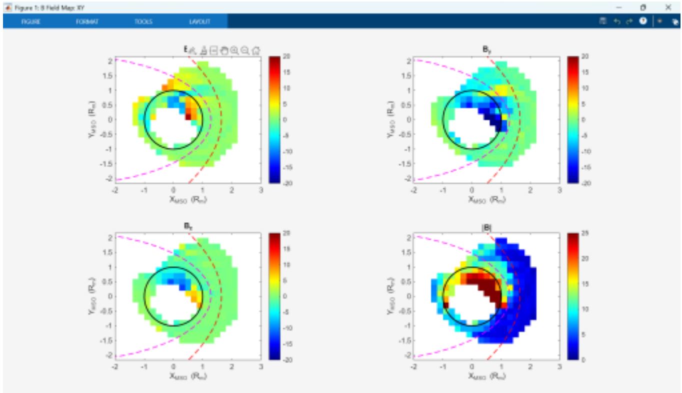
Magnetic field map in the XY plane, showing the magnetic field components ( B_x , B_y , B_z ) and magnitude ( |B| ) in nT.
