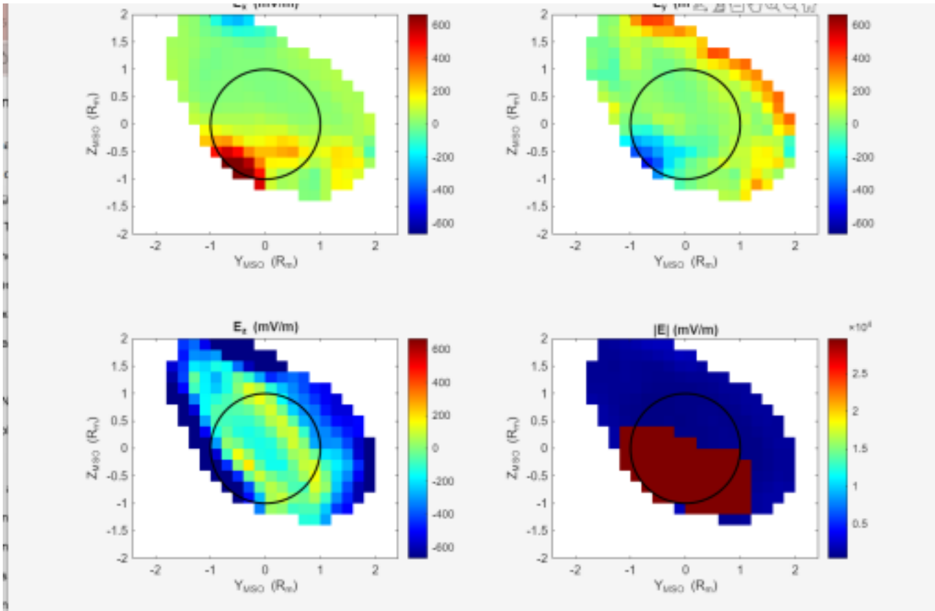
Convective electric field map in the YZ plane, showing E_x , E_y , E_z and |E| in mV/m. Description matched to the
