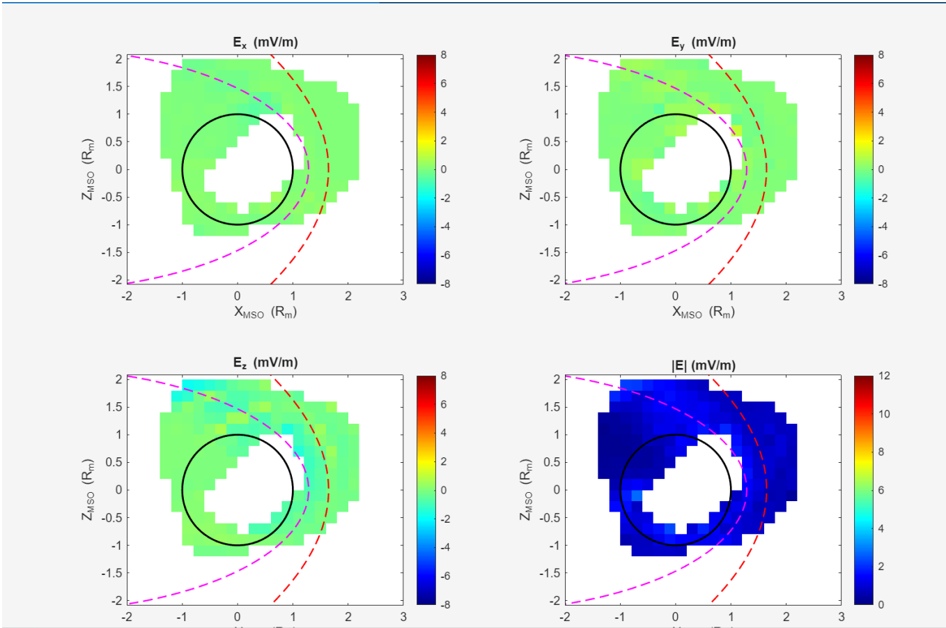
Convective electric field map in the XZ plane, showing E_x , E_y , E_z and |E| in mV/m. Description matched to the
