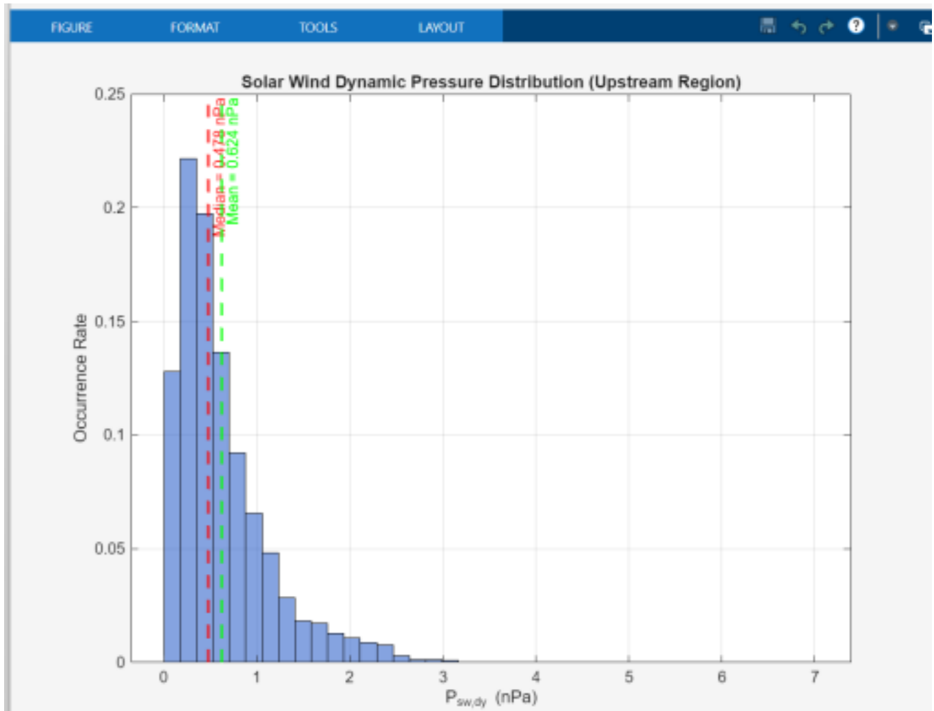
Solar-wind dynamic-pressure histogram for the upstream region, with median and mean markers. Description
