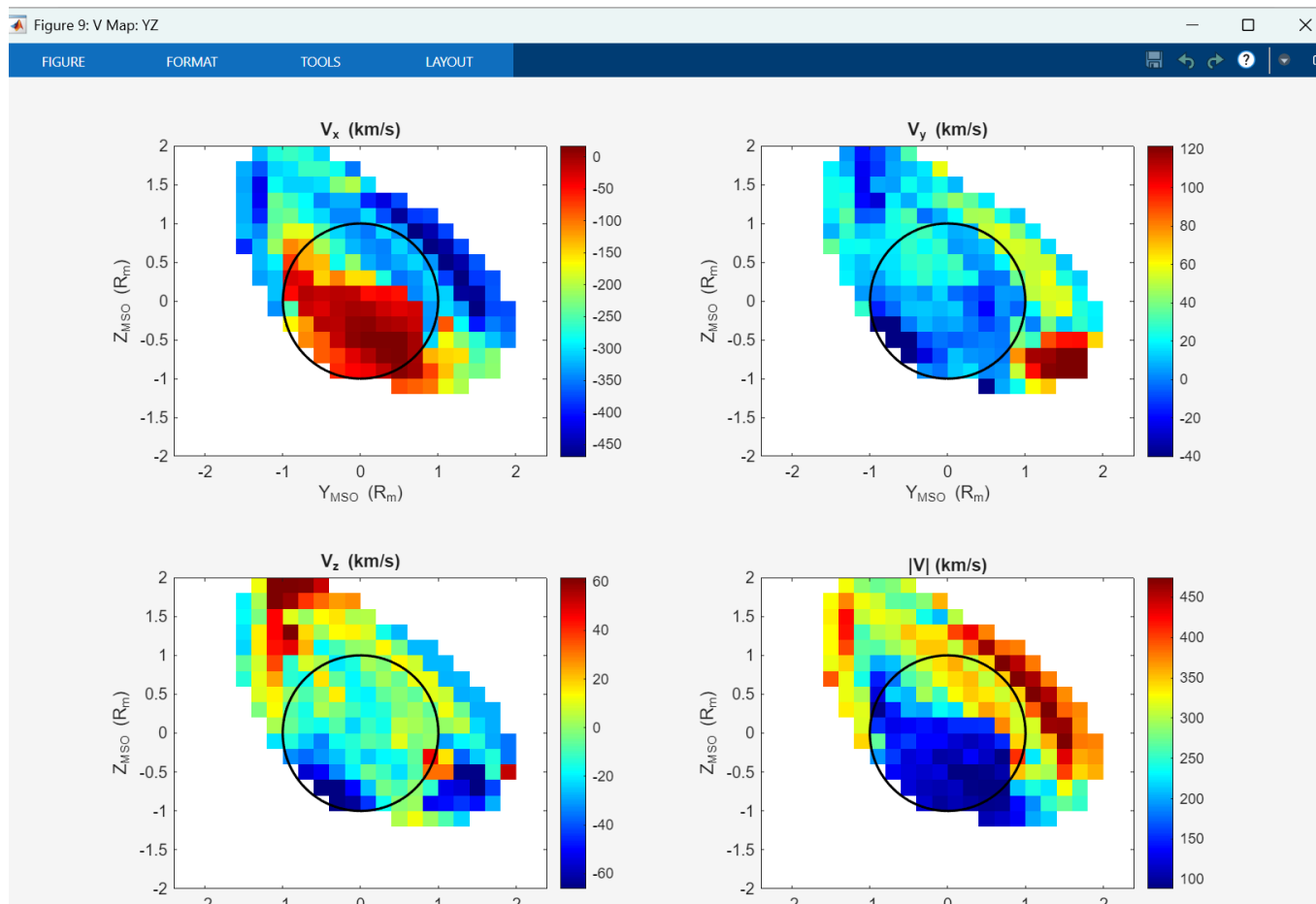
Alternate YZ-plane velocity capture, showing the four velocity components in the cross-tail projection.
