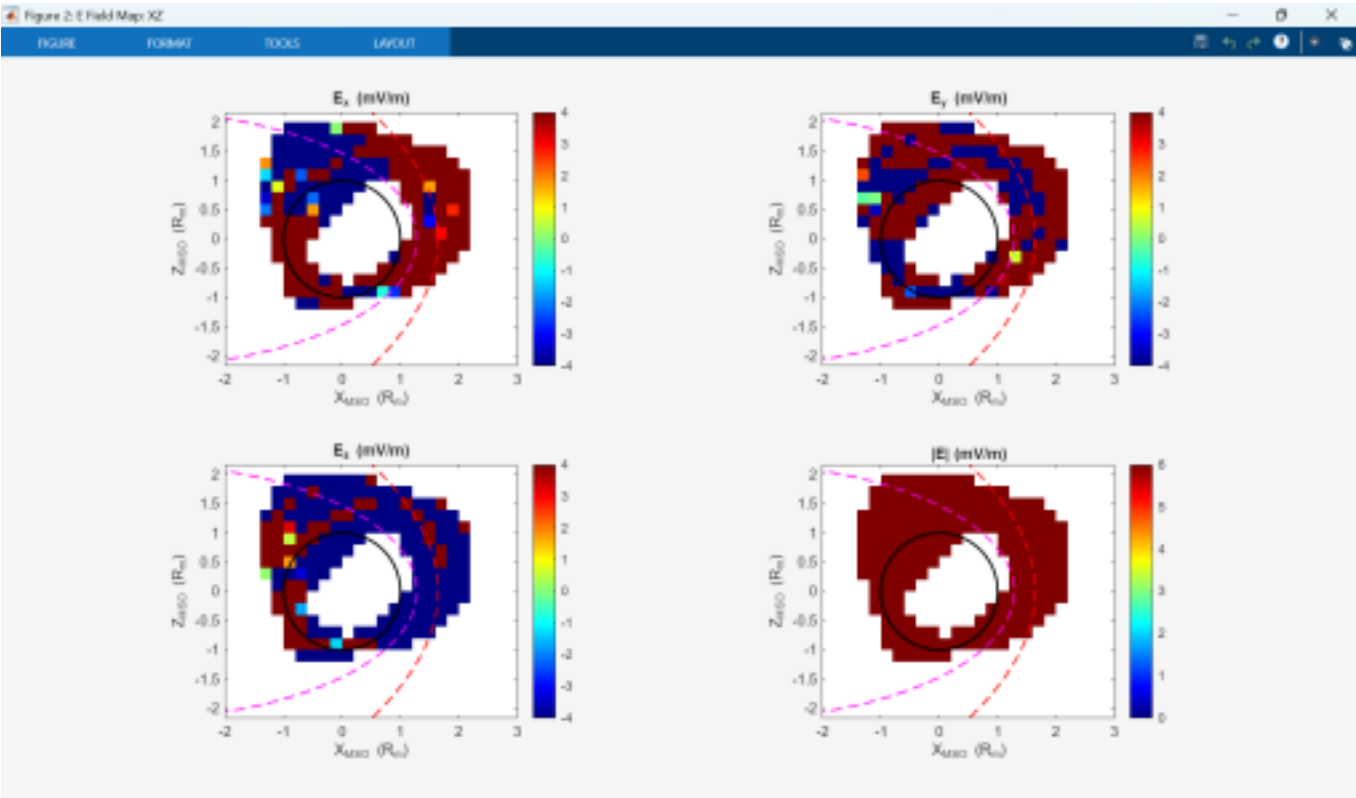
Convective electric field map in the XZ plane, showing E_x , E_y , E_z and |E| in mV/m. Description matched to the
