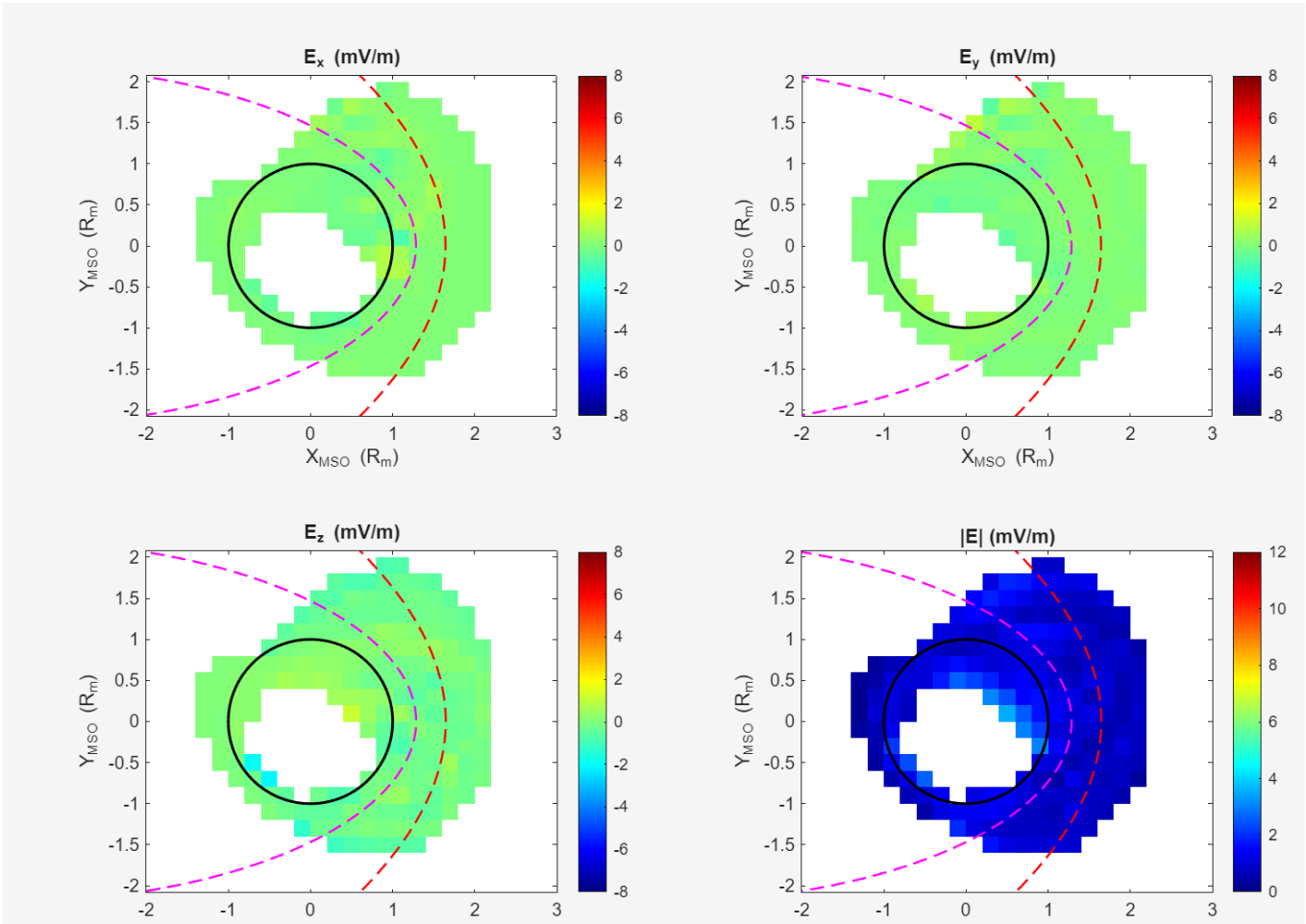
Convective electric field map in the XY plane, showing E_x , E_y , E_z and |E| in mV/m. Description matched to the
