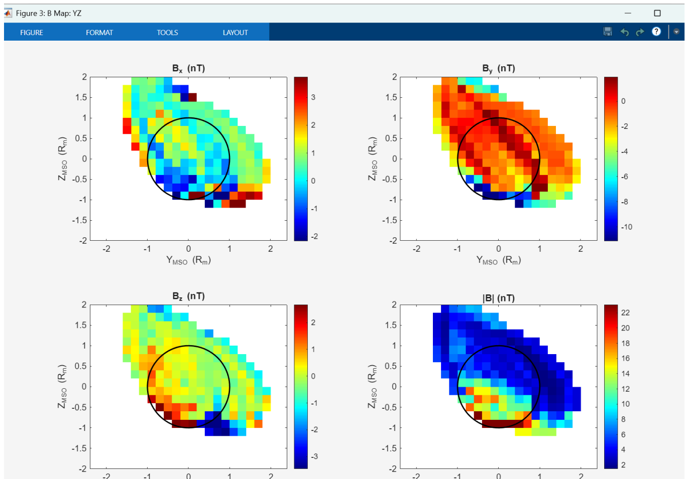
Magnetic field map in the YZ plane, showing B_x , B_y , B_z and |B| in nT.
