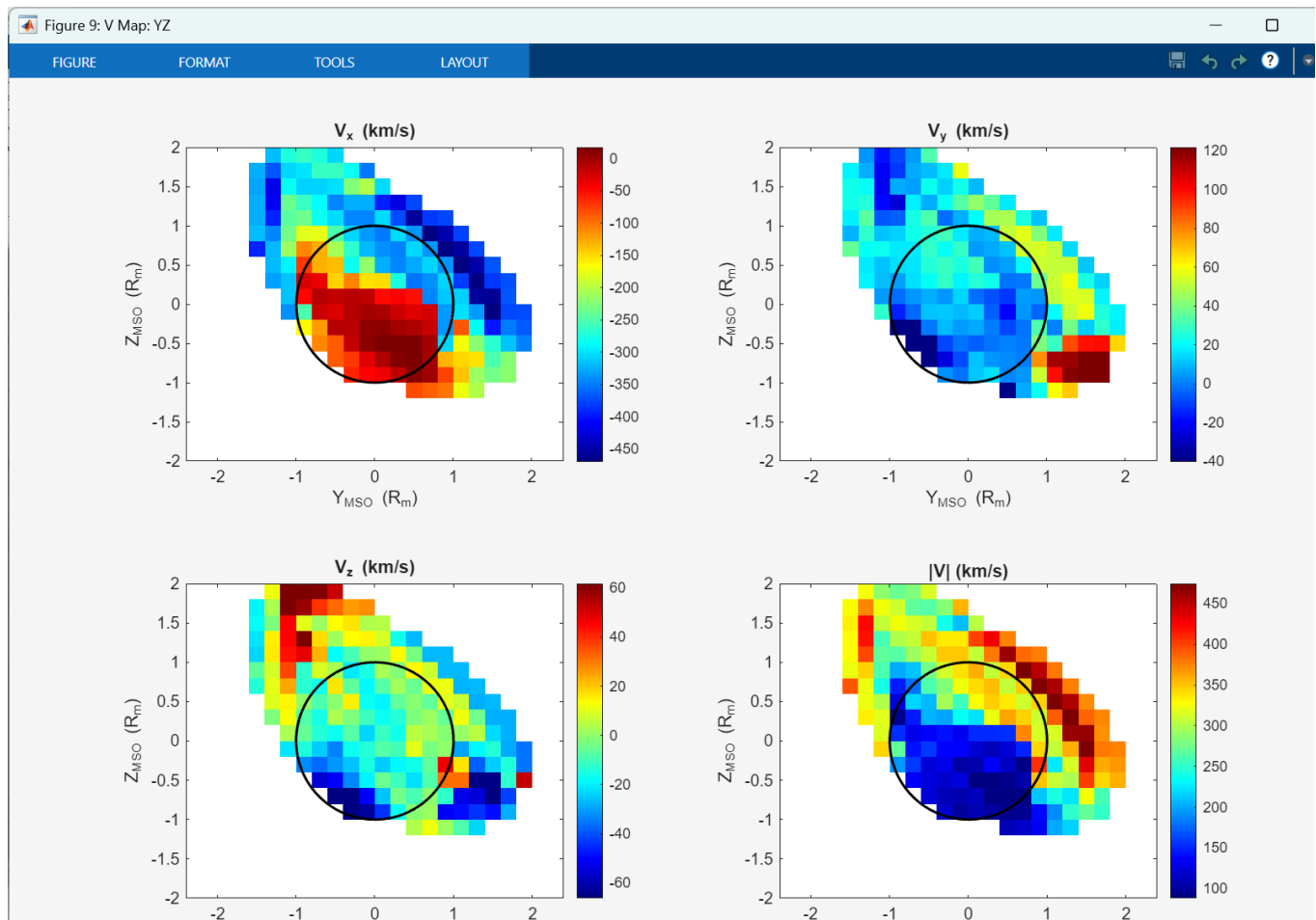
Velocity map in the YZ plane, showing V_x , V_y , V_z and |V| in km/s.
