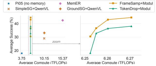
Figure 4. Efficiency-performance comparison among models.
