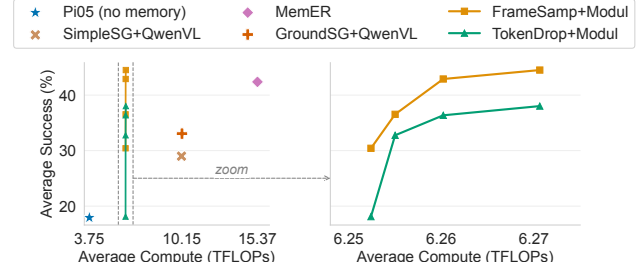
Figure 4. Efficiency-performance comparison among models.
