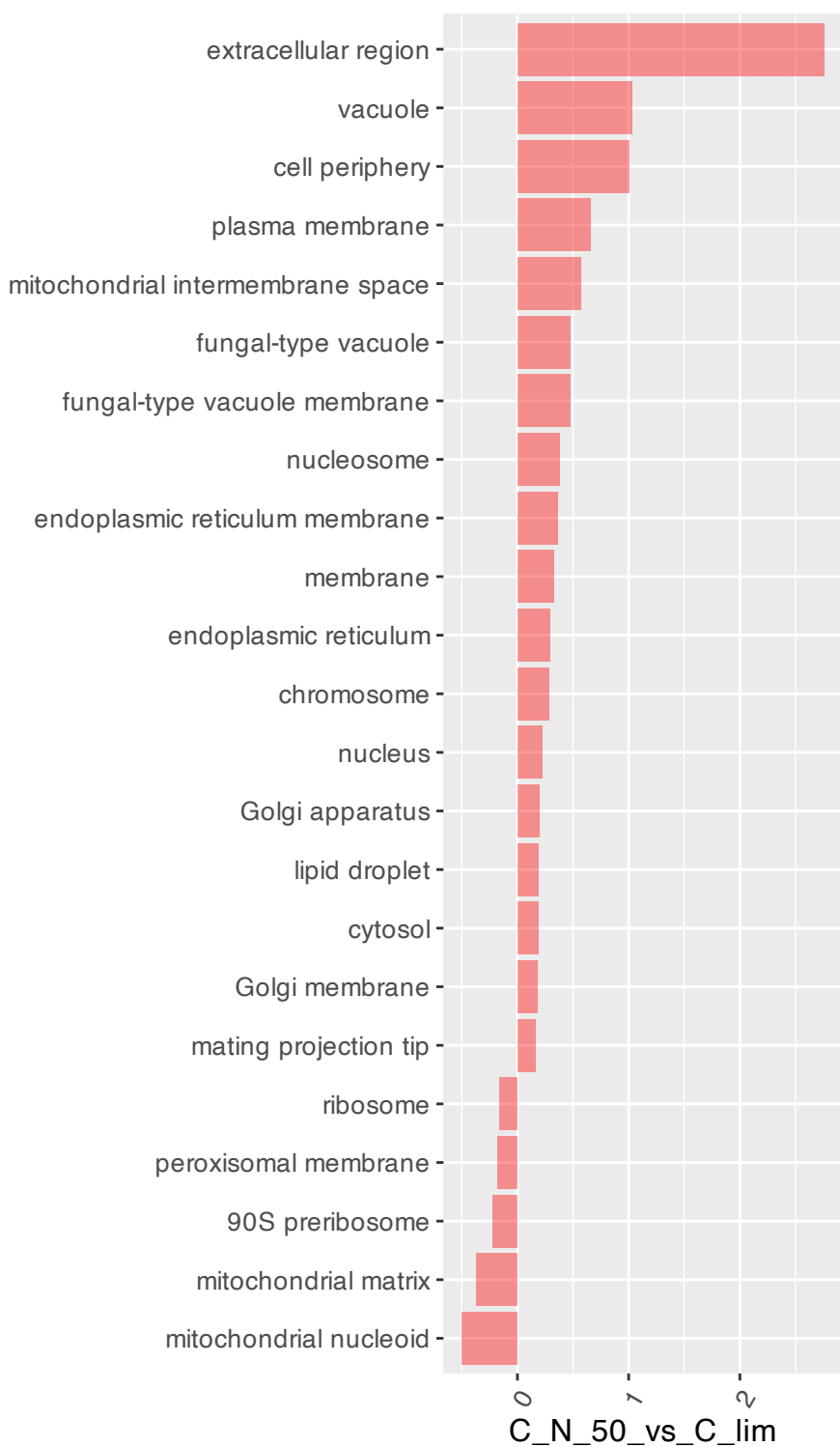
Cellular Component
