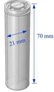
Fig. 2. A 21700-type battery cell in COMSOL.
