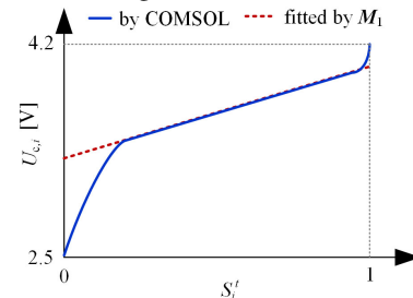
Fig. 4. Fitting the cell voltage profile using M_1 [6].
