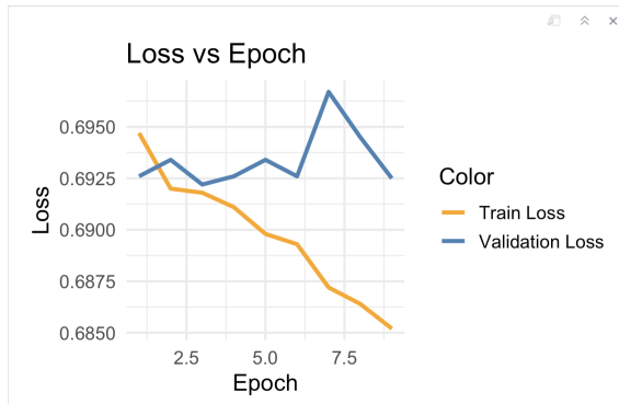
Figure 5: Loss
