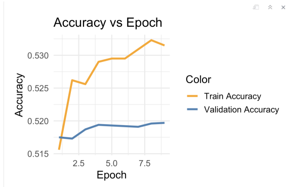
Figure 4: Accuracy
