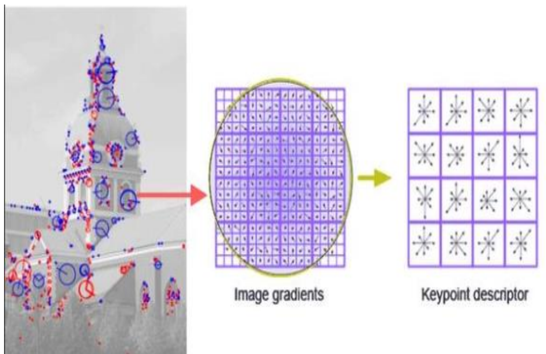
Figure 10 : SIFT-Coding [2]
