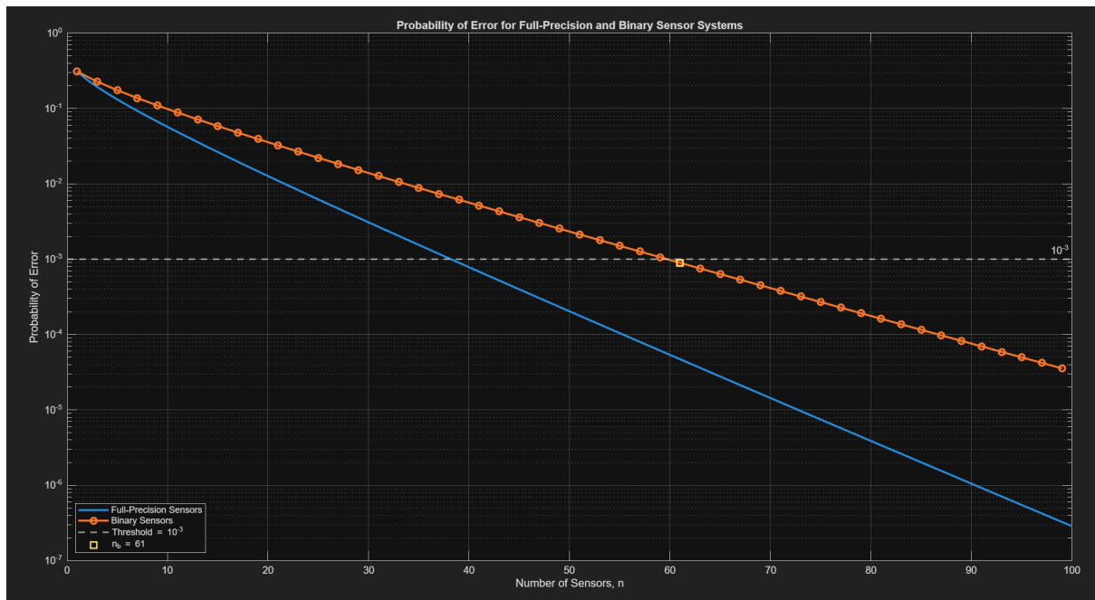
Figure 5: Probability of Error for Full-Precision and Binary Sensor Systems
