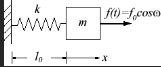
Figure 7.9: SDOF System forced by the harmonic function f(t) = f_0 \cos \omega t
