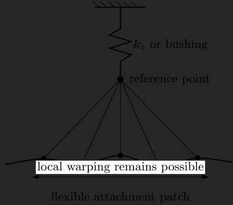
Figure 5.4: RBE3 used as a deformable distributed support. The interpolation maps the generalized motion of the flexible patch to a reference point; the spring or bushing supplies the actual stiffness. Modes lying in the null space of the interpolation are not directly stiffened by the support.
