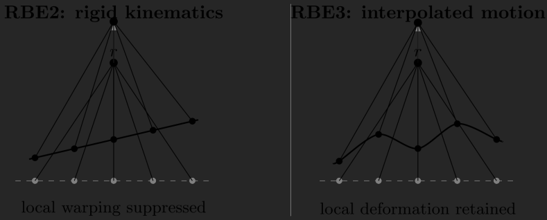
Figure 5.3: Conceptual difference between RBE2 and RBE3. The RBE2 prescribes the attachment-node motion from the reference motion and therefore suppresses relative deformation in the coupled DOFs. The RBE3 obtains a generalized reference motion from the attachment nodes, so local deformation modes can remain. The sketches are schematic rather than a literal depiction of a particular solver implementation.
