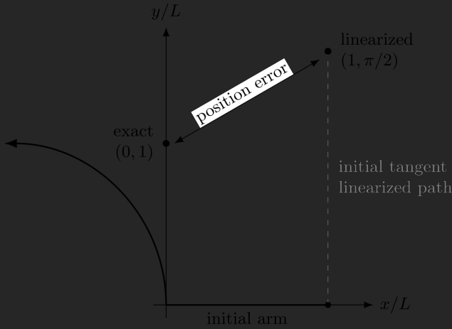
Figure 5.6: Finite rotation versus the small-rotation tangent approximation for a rigid arm. The exact dependent point follows a circular arc, whereas a constraint linearized in the initial configuration moves along the initial tangent. At 90^\circ the two positions are radically different.
