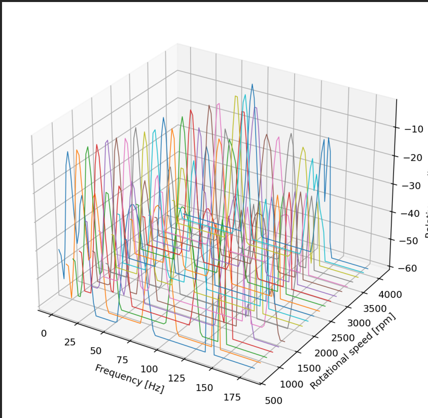
Figure 12.3: Waterfall representation of the synthetic response Campbell field. Each line is one spectrum at one rotational speed. The order-related peaks move in frequency, while the stationary 140 Hz component remains at the same frequency.
