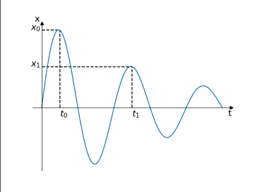
Figure 7.14: Determination of the damping ratio from the logarithmic decay
