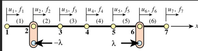
Figure 3.8: Physical interpretation of a Lagrange multiplier for u_2 = u_6 : the multiplier generates the equal-and-opposite reaction pattern required to enforce the relation exactly.
