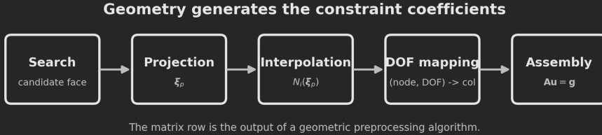
Figure 3.2: A surface-based constraint row is generated by a preprocessing pipeline: search identifies a candidate face, projection supplies local coordinates, interpolation supplies the coefficients, DOF mapping supplies the global columns, and assembly finally creates the algebraic constraint.
