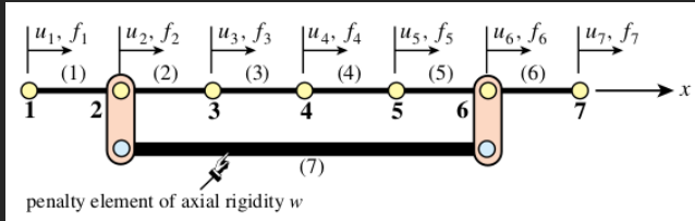
Figure 3.7: Penalty interpretation of u_2 = u_6 : a fictitious high-stiffness element penalizes relative motion.
