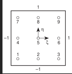
Figure 11.1: Integration points for n = 3 in a square region. Exact for a polynomial of fifth order in each direction
