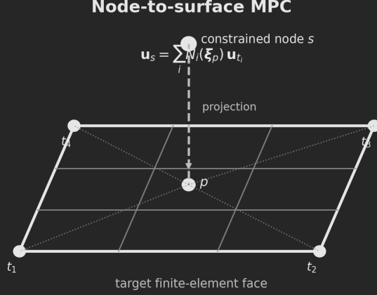
Figure 3.3: Node-to-surface MPC. The constrained node is projected onto a target finite-element face. The target shape functions evaluated at the projected point provide the coefficients that relate the constrained-node motion to the target nodal DOFs.
