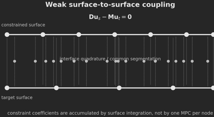
Figure 3.5: Weak surface-to-surface coupling between nonmatching meshes. A common interface segmentation supplies quadrature points. Contributions from both interpolation fields are integrated into the matrices \mathbf{D} and \mathbf{M} , producing \mathbf{D}\mathbf{u}_s - \mathbf{M}\mathbf{u}_t = \mathbf{0} .
