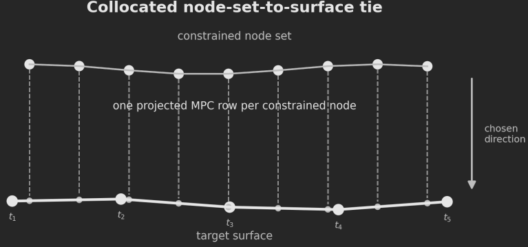
Figure 3.4: Collocated node-set-to-surface tying. Every constrained node is projected independently onto the target surface and generates its own MPC row. The discretization is therefore directional and depends on which side is selected as the constrained node set.
