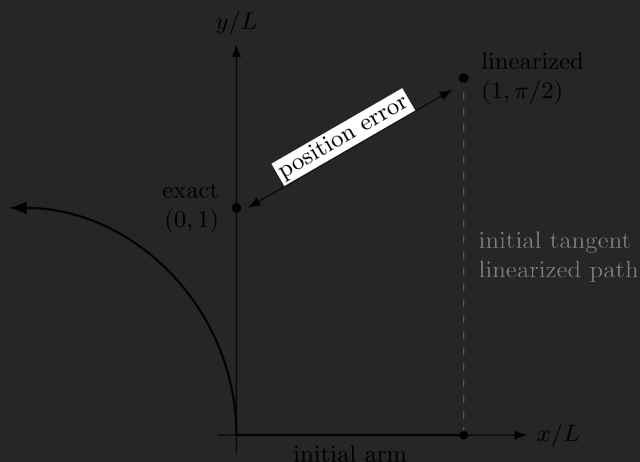
Figure 5.4: Finite rotation versus the small-rotation tangent approximation for a rigid arm. The exact dependent point follows a circular arc, whereas a constraint linearized in the initial configuration moves along the initial tangent. At 90^\circ the two positions are radically different.
