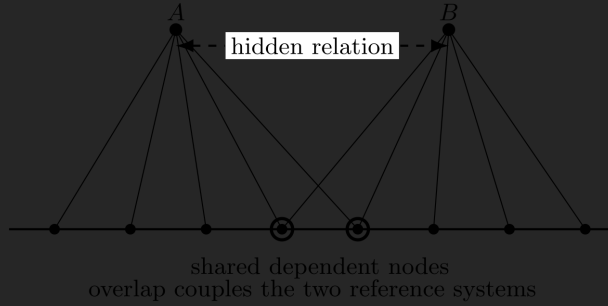
Figure 5.5: Overlapping RBE2 spiders. A node that is dependent on both reference systems must satisfy both rigid-body relations simultaneously. The overlap therefore introduces an implicit relation between reference points A and B ; enough shared nodes can effectively merge the two spiders into one rigid region.
