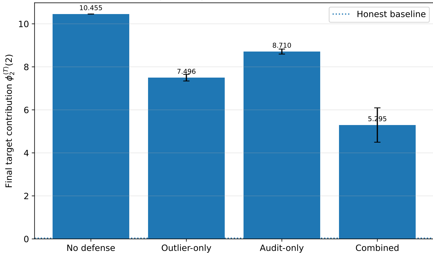
Figure 6: Byzantine collusion attack
