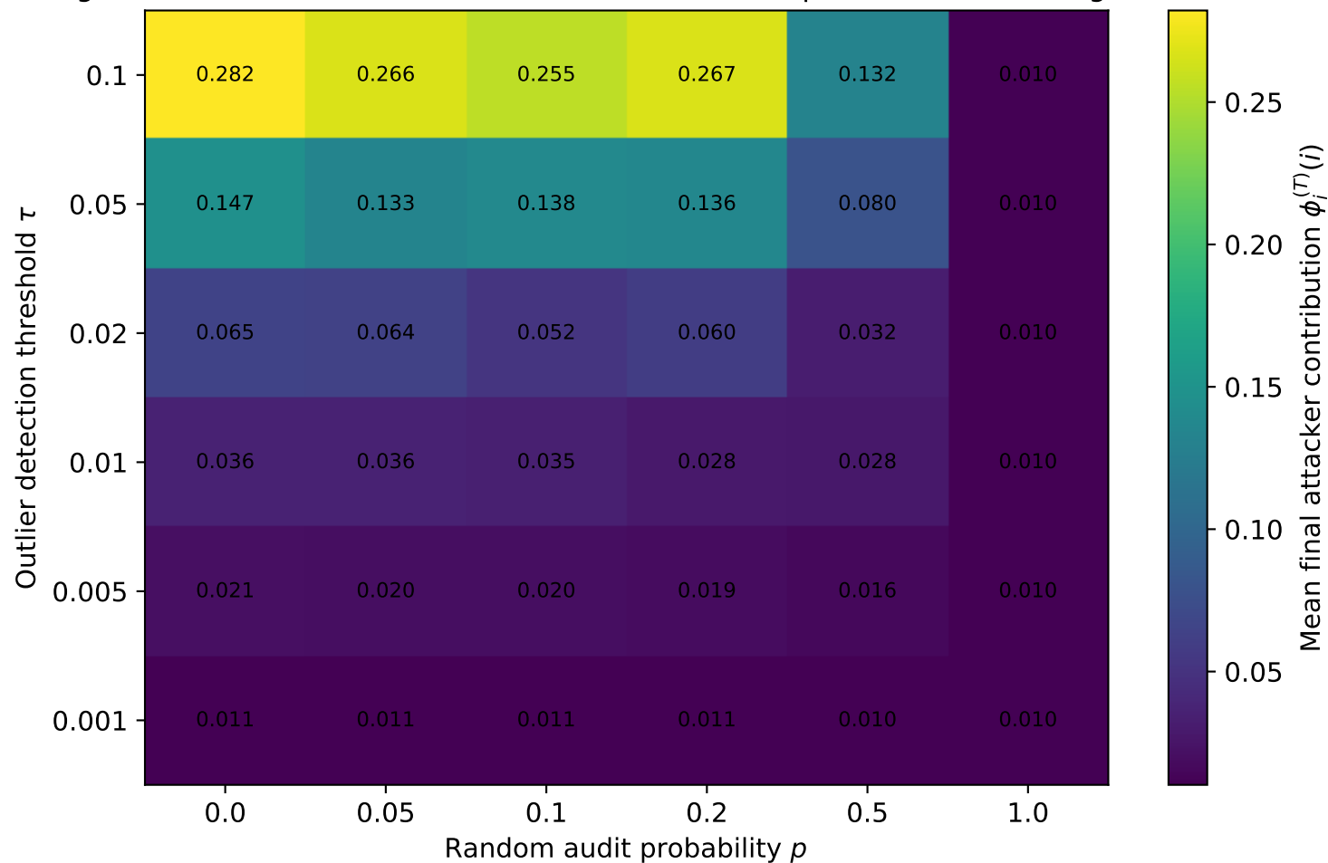
Figure 7: Interaction between outlier detection and probabilistic auditing (RQ3)
