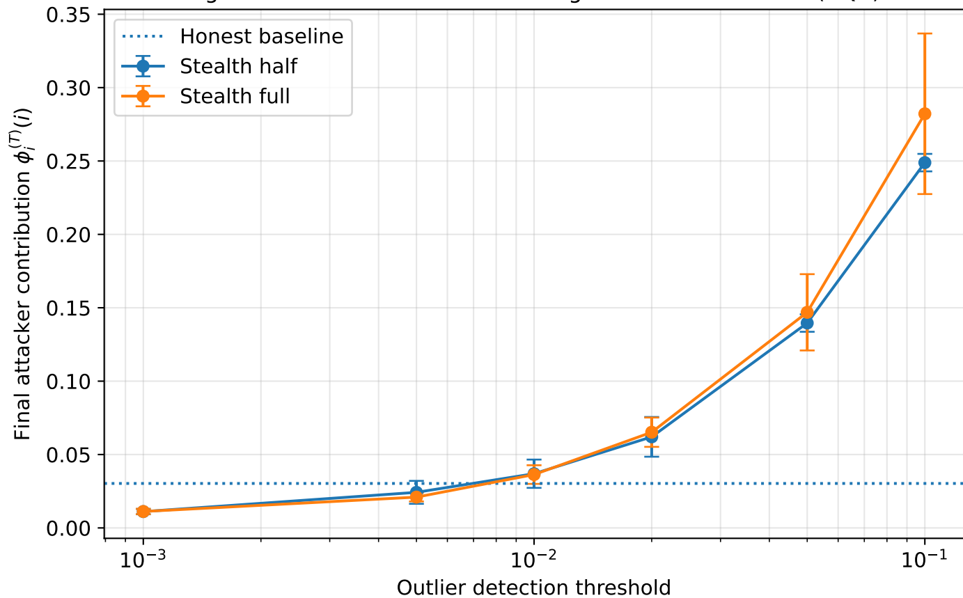
Figure 2: Outlier detection alone against stealth attacks (RQ3)
