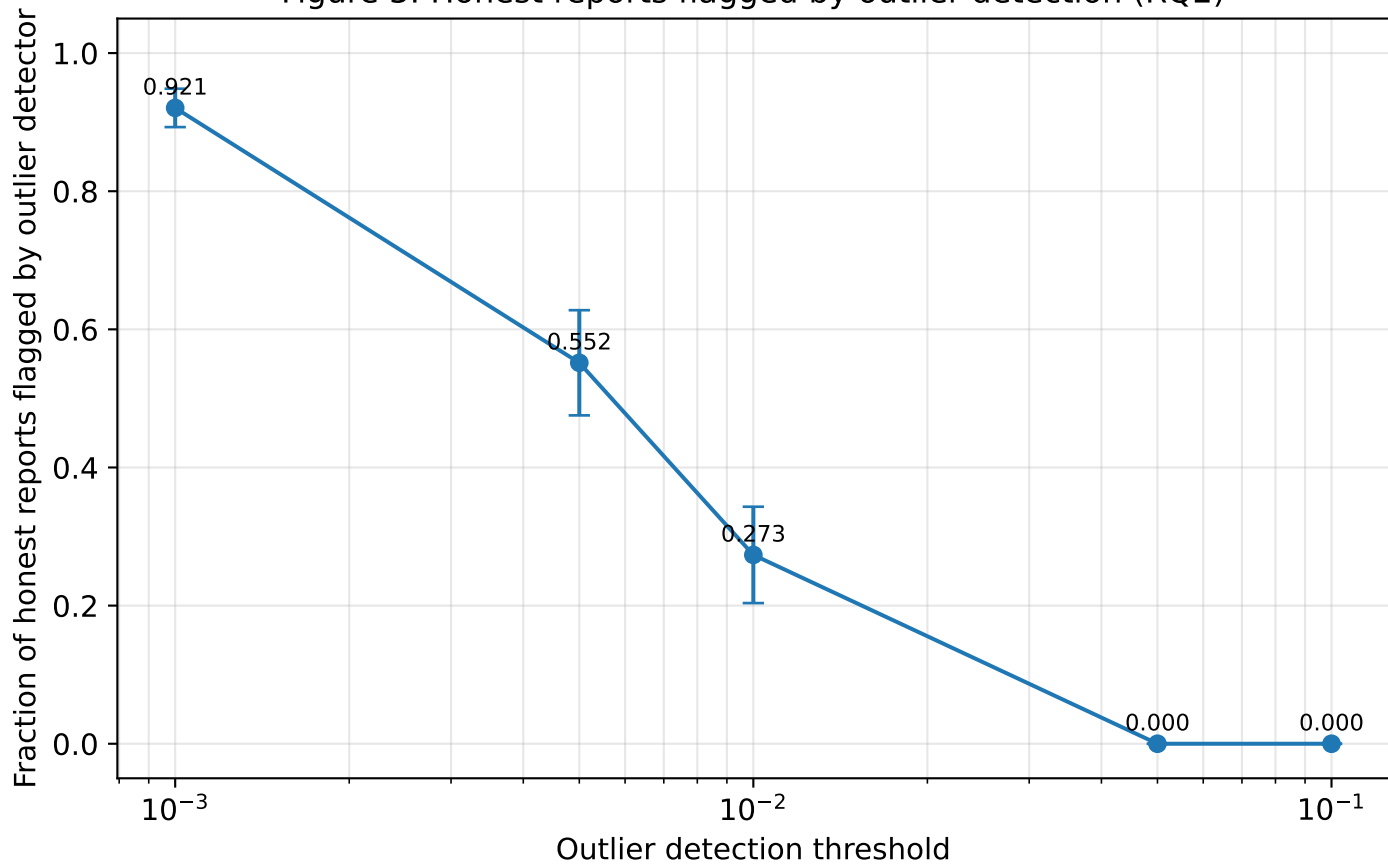
Figure 3: Honest reports flagged by outlier detection (RQ2)
