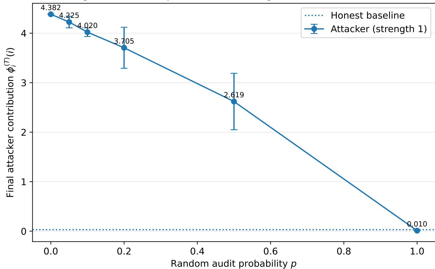
Figure 4: Effect of probabilistic auditing on attack reward (RQ3)
