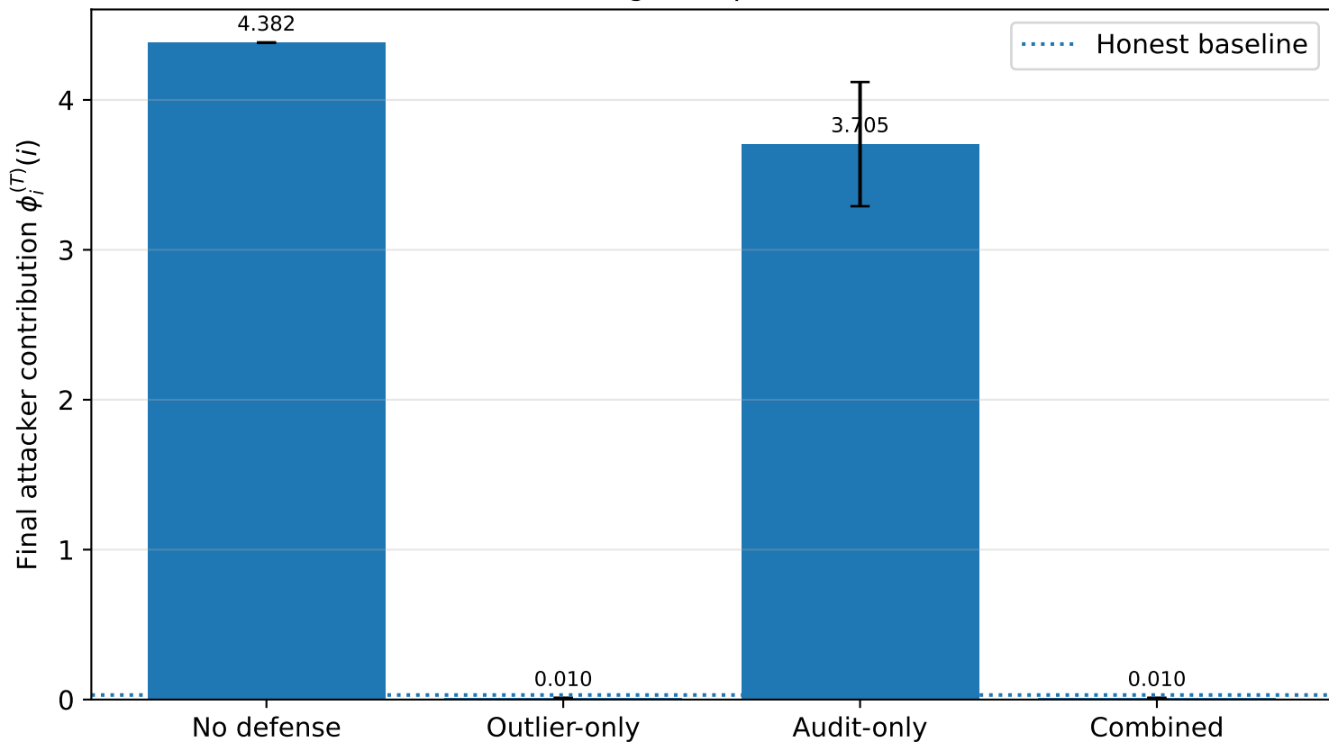
Figure 5: Comparison of defense configurations (RQ3) Fixed attack (strength 1), p=0.2 , threshold=0.01
