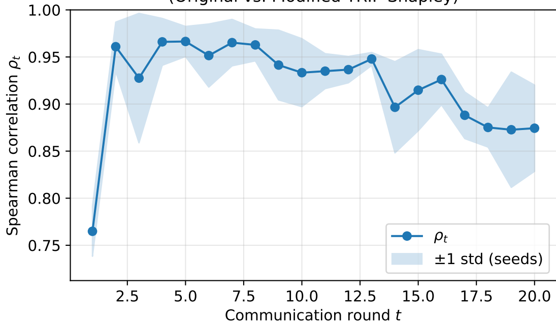
Honest scenario: ranking correlation (Original vs. Modified TRIP-Shapley)
