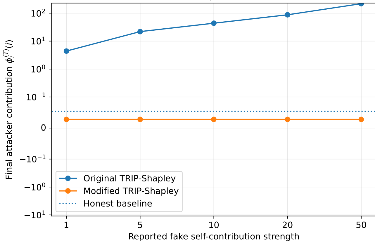
Attack effectiveness (p=0.2, threshold=0.01)
