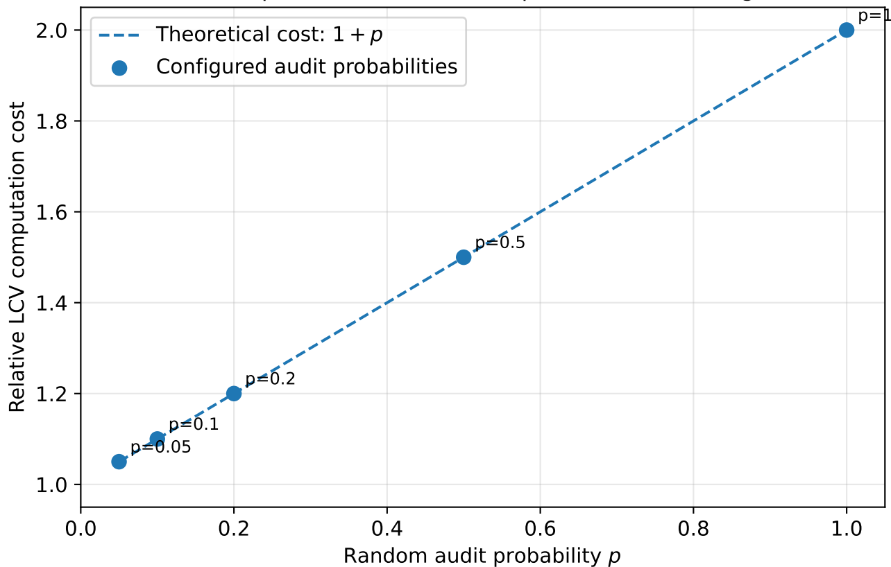
Computational overhead of probabilistic auditing
